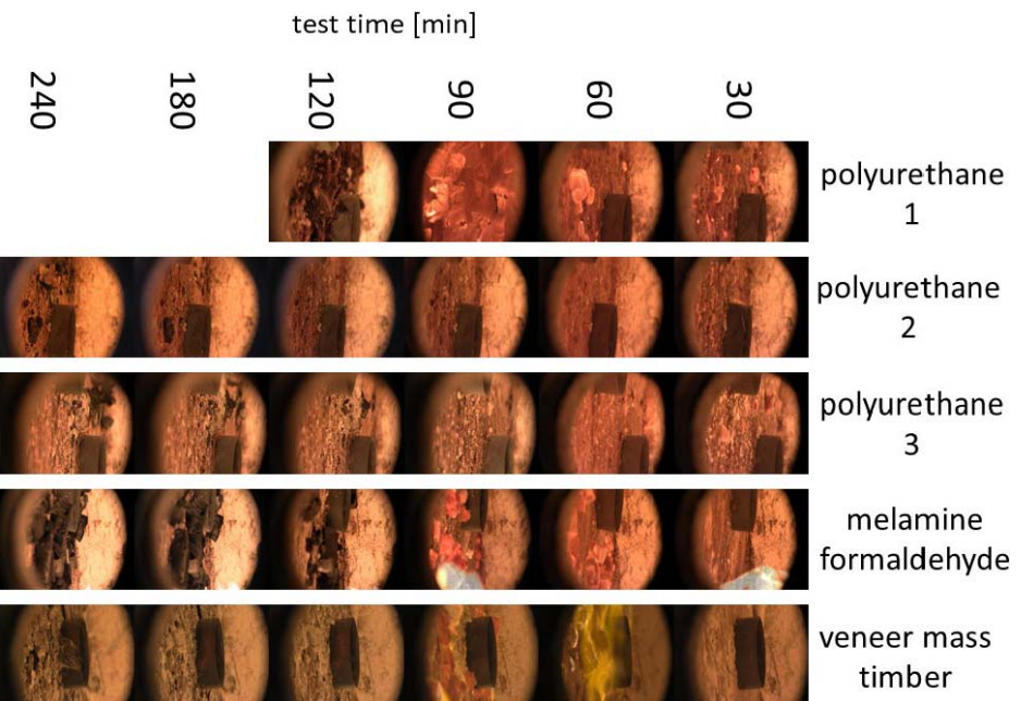
Figure 5.—Images of the furnace floor during the test showing that charred wood dropped from the specimen during the test from a representative sample.
