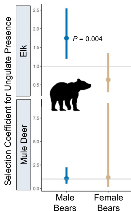
FIGURE 4 Selection coefficients ( \exp[\beta_{\text{ungulate presence}}] ) from step-selection functions assessing whether male and female black bears made movements that placed them in a 200-m proximity of parturient mule deer or elk more often than expected by chance in northeastern Oregon, 2016–2019. Dots represent point estimates for the selection coefficient for mule deer or elk presence and bars represent 95% confidence intervals. The gray horizontal line at y = 1 indicates indifference toward parturient elk; values above this line indicate selection and values below the line indicate avoidance. p -values indicate whether the parameter differed significantly from zero.
