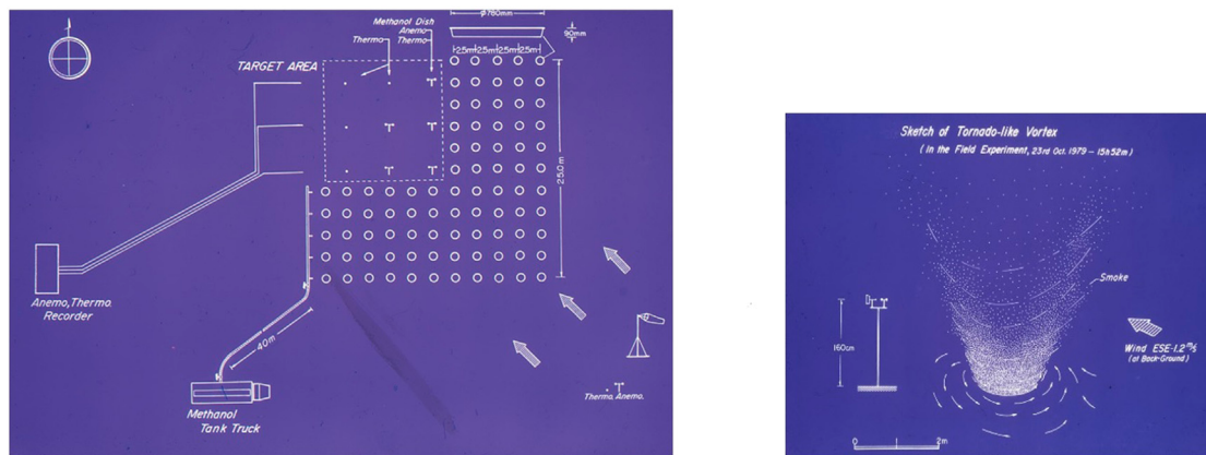
FIGURE 6 Schematic of 1/100 scale model outdoor fire whirl experiment and type 3 fire whirl.
