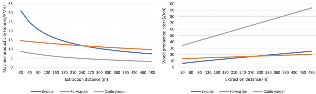
Figure 7. Productivity and production cost of three different extraction machines depending on average skidding distance from the ThinCost_1.0 for round-wood only.
