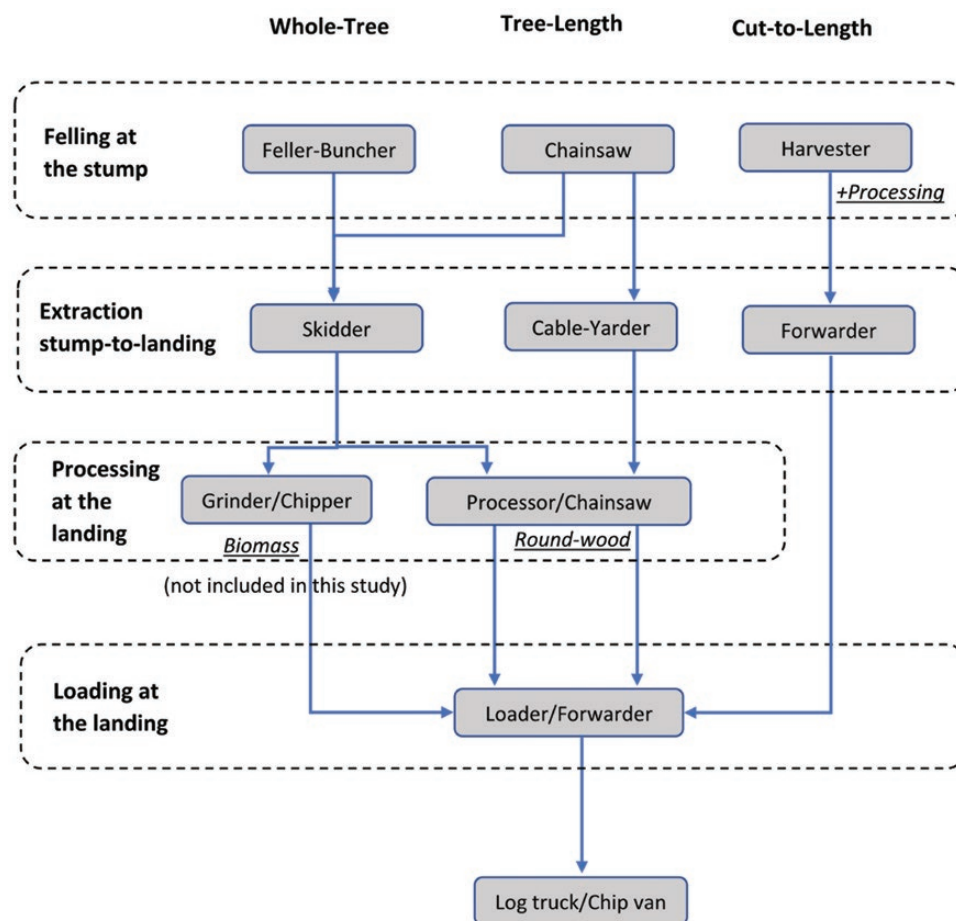
Figure 1. Three forest harvesting methods that are commonly used in forest thinning operations. Biomass: wood chips, wood slash, and residues from the harvesting process.
