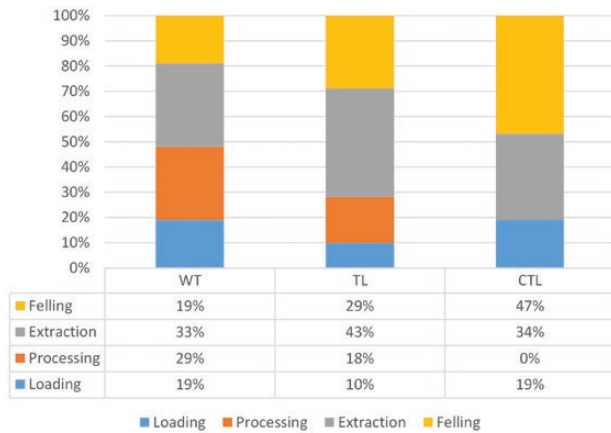
Figure 3. The ratio of each phase (felling, extraction, processing and loading) of thinning operation to total stump-to-truck harvesting cost. CTL ( n=8 ), TL ( n=2 ), WT ( n=10 ), Felling in CTL includes felling and processing. Processing activity in the CTL harvesting system is included in the felling activities.
