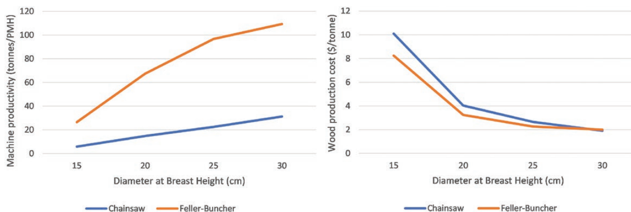
Figure 6. Productivity and cost of felling machine over different size of trees from ThinCost_1.0 model for harvesting roundwood only.
