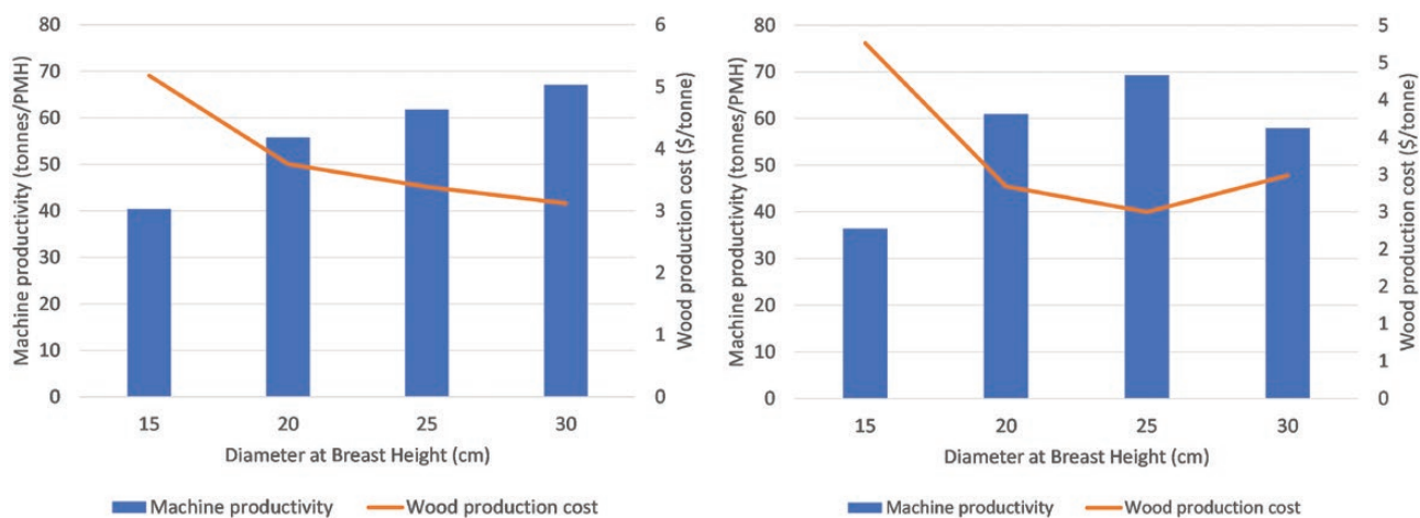
Figure 8. Productivity and production cost of processor (left) and loader (right) depending on DBH from the ThinCost_1.0 for round-wood only.
