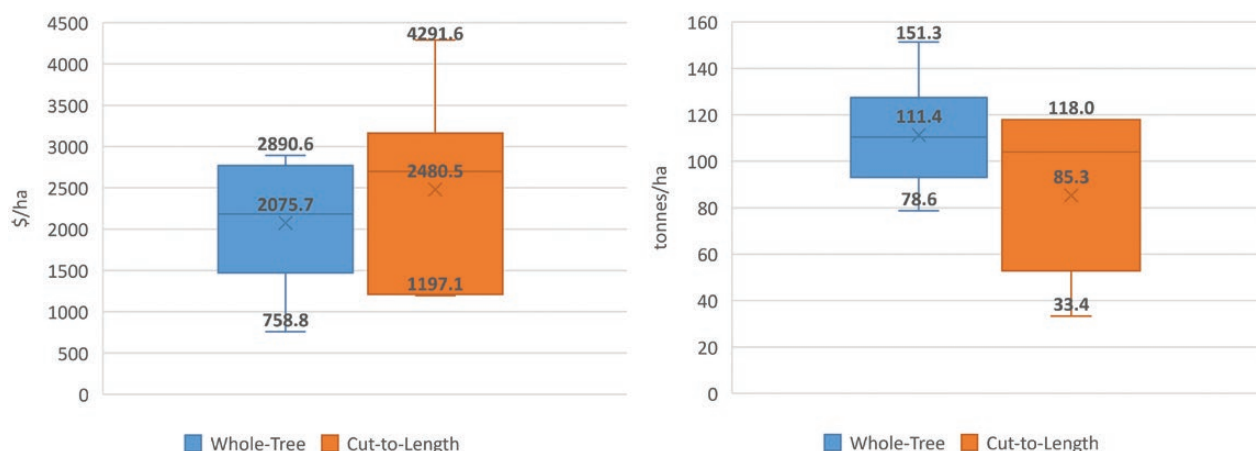
Figure 5. Average costs ($/ha) of thinning operations and harvested volume (tons/ha) from the reviewed papers. Harvested volumes include both roundwood and biomass in whole-tree and roundwood only in cut-to-length thinning operations.
