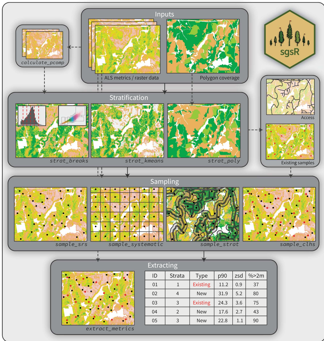
Figure 1 sgsR processing workflow detailing potential inputs, a selection of stratification and sampling algorithms, and supplementary processing strategies.
