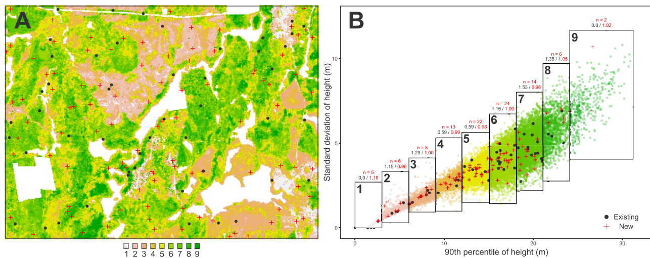
Figure 6 Example 2 processing outputs. Map of quantile strata (A) with existing (black) and new (red) sample units. Scatter plot (B) with quantile delineations by color and black boundaries. Existing and new sample units are presented to indicate their location within the distribution of the 90 th percentile of height and standard deviation of height. Text above quantile boundaries denotes the initial existingRatio of sample units (black) and samplingRatio following addition of new sample units (red). The number of sample units added to each quantile is listed for each quantile (e.g. n = 2 ).
