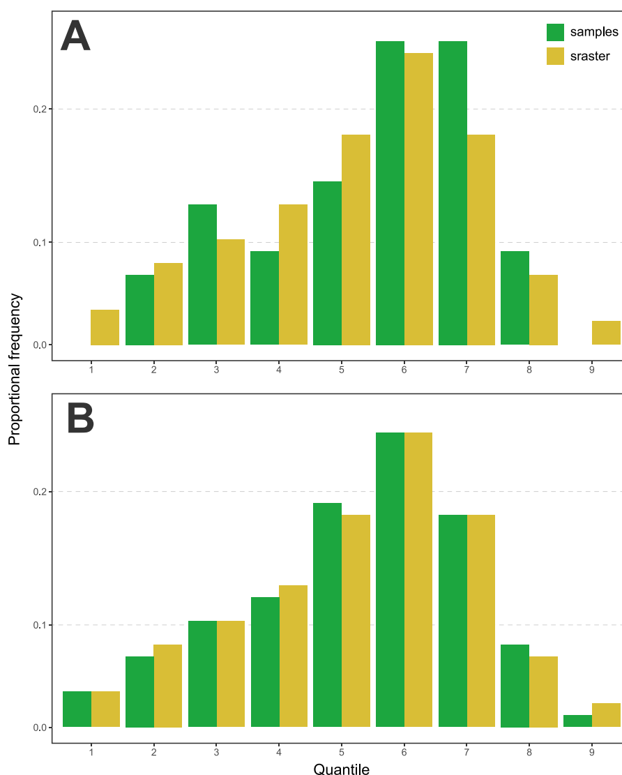
Figure 7 The sampling frequency (green) and stratum coverage frequency (yellow) for existing sample units only (A) and existing and new sample units (B) for the 90 th percentile of height. Bars with an unequal value for a given quantile indicate that the number of sample units and the coverage of the strata are not proportional.
