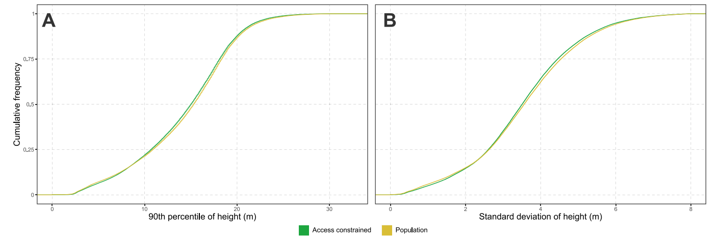
Figure 4 Cumulative frequency distributions for zq90 (A) and zsd (B) that compare the access constrained region (green) with populations (yellow).
