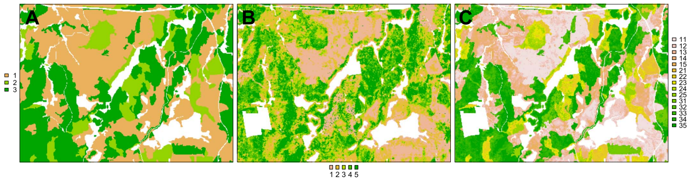
Figure 3 Stratification into three classes using strat_poly (A); 5 class p90 stratification derived using strat_quantiles (B); mapped combination of strata from A and B derived using strat_map (C). Mapped raster stratum indices combine to form the final stratum values (e.g. stratum A1 and B1 combine to make C11).
