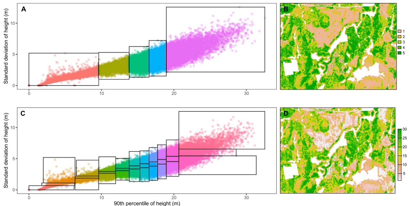
Figure 2 Single (90 th percentile of height) and dual (90 th percentile of height and standard deviation of height) stratification scatter plots (A and C, respectively) and rasters (B and D, respectively) colored to distinguish classes and delineated with black boundaries. Stratifications were generated using the strat_quantiles function in sgsR .
