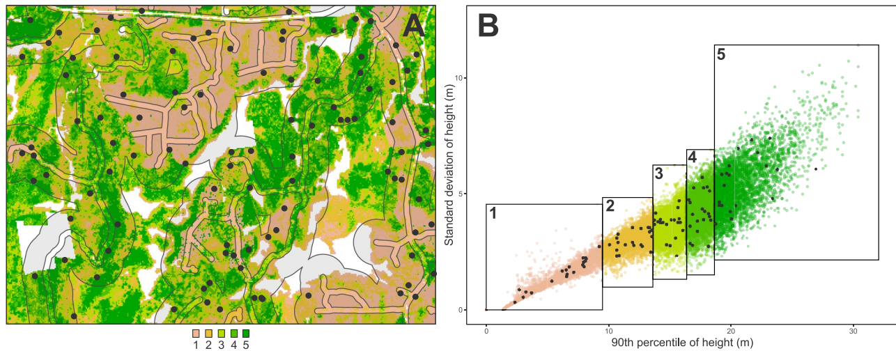
Figure 5 Graphical result of sampling from Example 1 with mapped sample units and road access buffers (A), and scatter plot showing distribution of sample units (black) in relation to the overall population (colored by strata; B). Stratification was performed on zq90 only. The scatter plot with zsd on the y-axis is purely to enable visualization.
