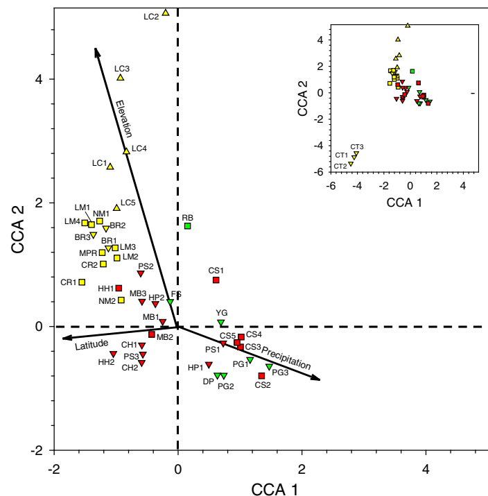
Figure 3 Canonical correspondence analysis plot of 44 sites sampled during 2016–2017 survey period. See Table 2 for site abbreviations. Symbol shapes refer to elevation classes arbitrarily chosen for illustration purposes: 580–600 m (upward pointing triangles), 60–240 m (squares), and <60 m (downward pointing triangles) (see Table S2 for latilong, elevation, and precipitation values for each site). Symbol colors refer to three precipitation classes arbitrarily chosen for illustration purposes: relatively low (yellow), intermediate (green), and relatively high (red) precipitation. The inset shows all sites in the larger figure along with the three CT sites in the lower left. Full-size DOI: 10.7717/peerj.14928/fig-3
