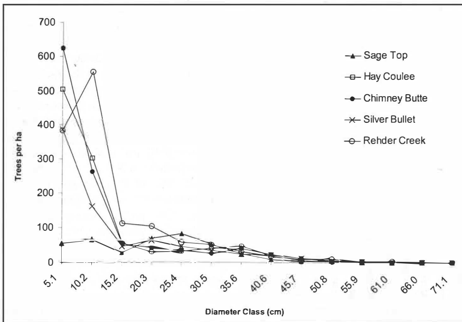
Figure 1. Diameter distribution of trees > 5.0 cm at the Bull Mountains old-growth ponderosa pine sites.
