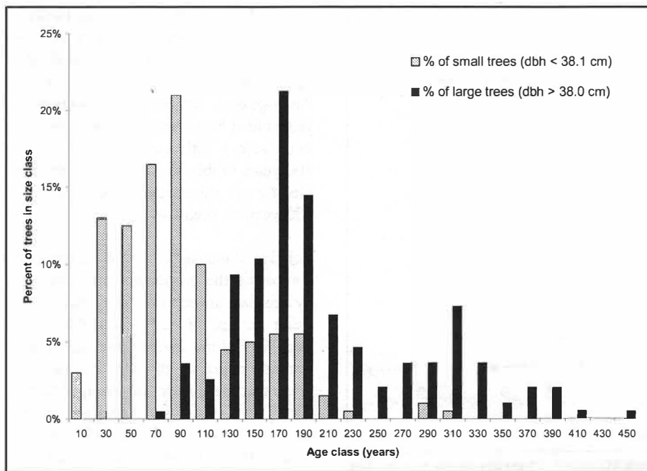
Figure 2. Percent of aged large and small trees by 20-year age classes across the Bull Mountains old-growth ponderosa pine sites.
