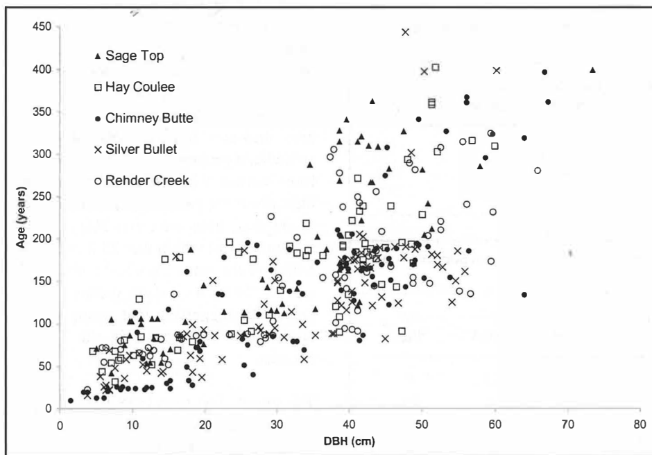
Figure 3. Tree age at breast height vs. diameter at breast height for Bull Mountains old-growth ponderosa pine sites.
