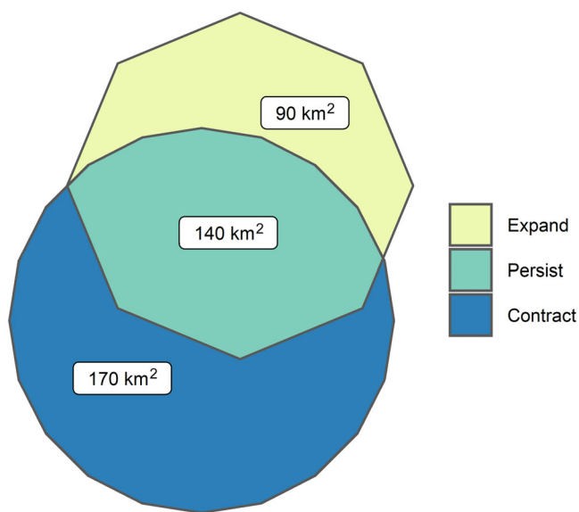
FIGURE 2 Conceptual relationship between the area of range contraction, persistence, and expansion. In this example, the current range size was 310 km 2 (i.e., sum of range persistence and contraction area) and the future range size was 230 km 2 (sum of range persistence and expansion area).
