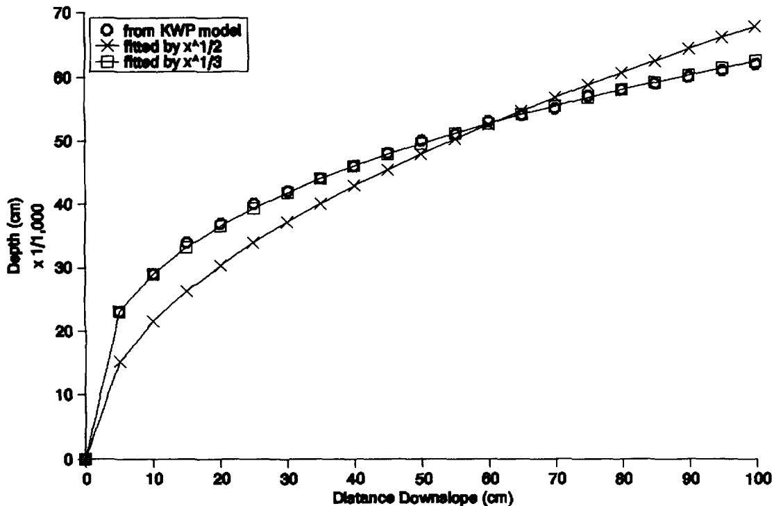
Fig. 3. Water surface profile calculated by kinematic wave-Philip model compared to best fit by the equations \epsilon x^{1/2} and \epsilon x^{1/3} .
