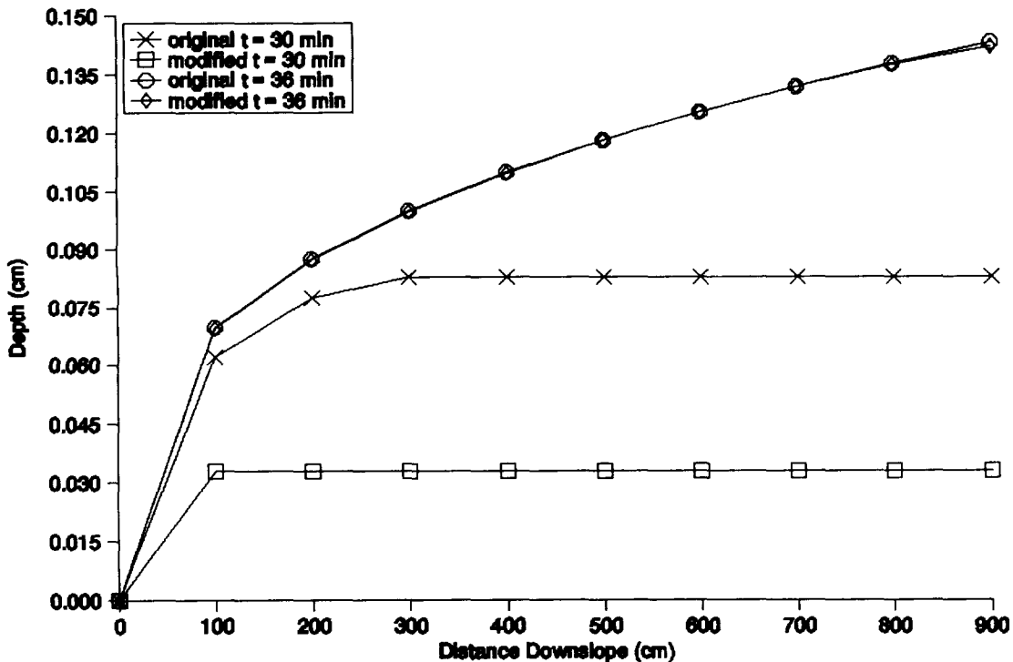
Fig. 6. Rising stage water surface profiles from the original and modified model.
