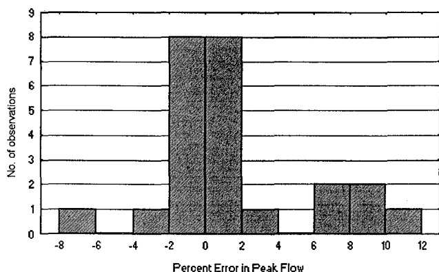
Figure 11. Distribution of percent error for predicted hydrographs at Tea Meadow.
