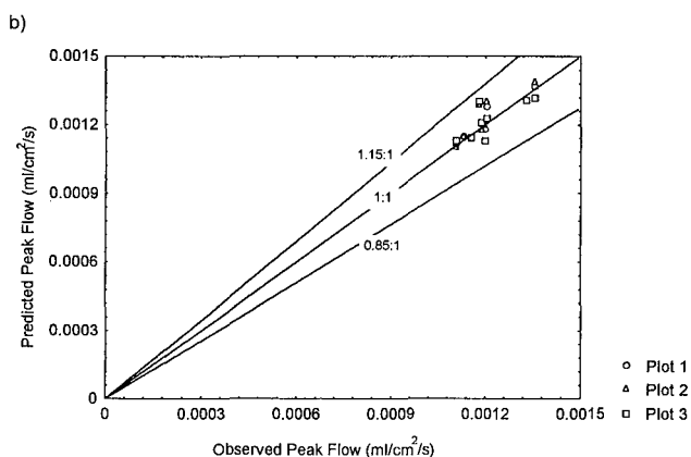
Figure 12. Predicted versus (a) observed runoff volumes and (b) peak flows.
