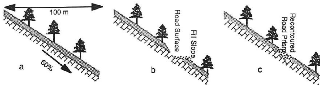
Figure 1. Section of Hillslope With 60 Percent Slope a) With Undisturbed Forest; b) With a Road; and c) Following Recontouring of the Road.
