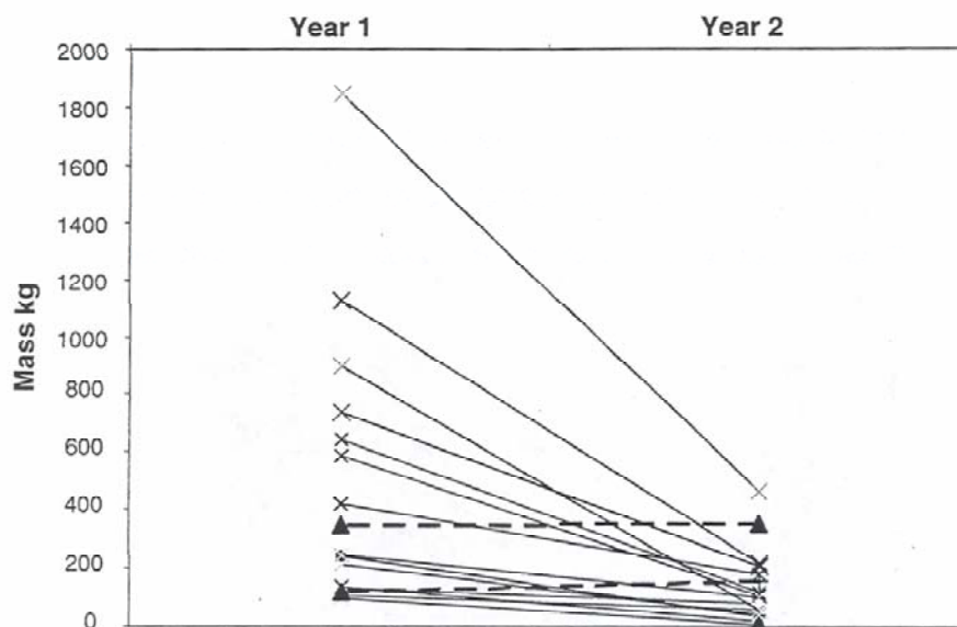
Figure 1. Mass of sediment from plots with road, cutslope, and ditch disturbed in the first year, and recovering in the second year. The average interannual decline is 72 percent. The two plots, which showed an increase of 12 percent, are shown with dashed lines.
