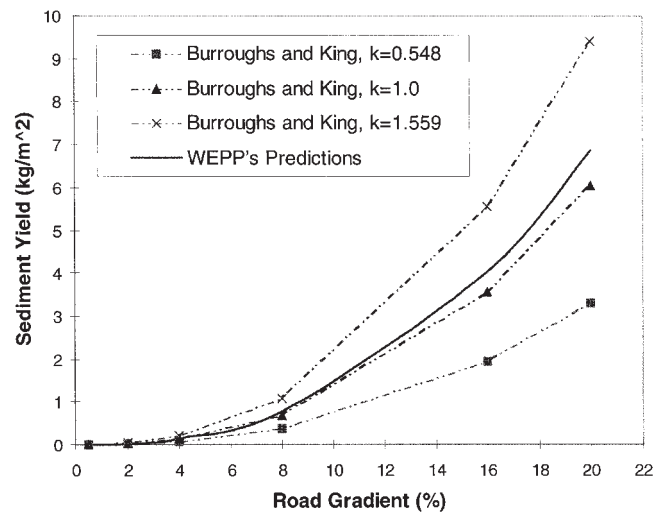
FIGURE 5 Average annual sediment yield using Burroughs and King (12) equation and WEPP's predictions for similar soil and climate.
