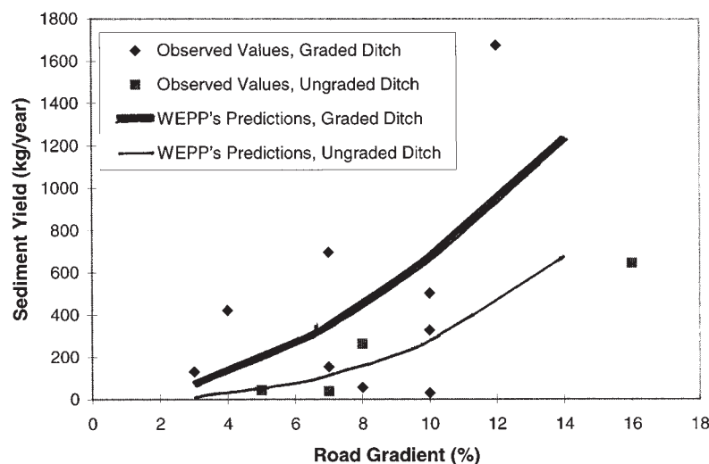
FIGURE 1 Average annual measured and predicted sediment yields for 60-m-long road (5).
