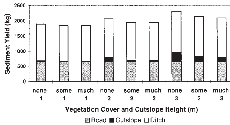
FIGURE 6 WEPP's predicted sediment yield for different cutslope heights and vegetation amounts for 1 year for watershed consisting of 4 percent silt loam road 60 m long, with channel and cutslope.
