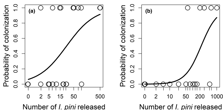
FIGURE 3 Colonization rates of Ips pini in relation to numbers of propagules released (log scale) in (a) 1 m caged and (b) 10 m field scenarios. Colonization was defined as at least one billet out of four per release replicate having at least one F1 adult present. Each data point represents one release replicate. A binomial generalized linear model was fit to the data to produce each line.
