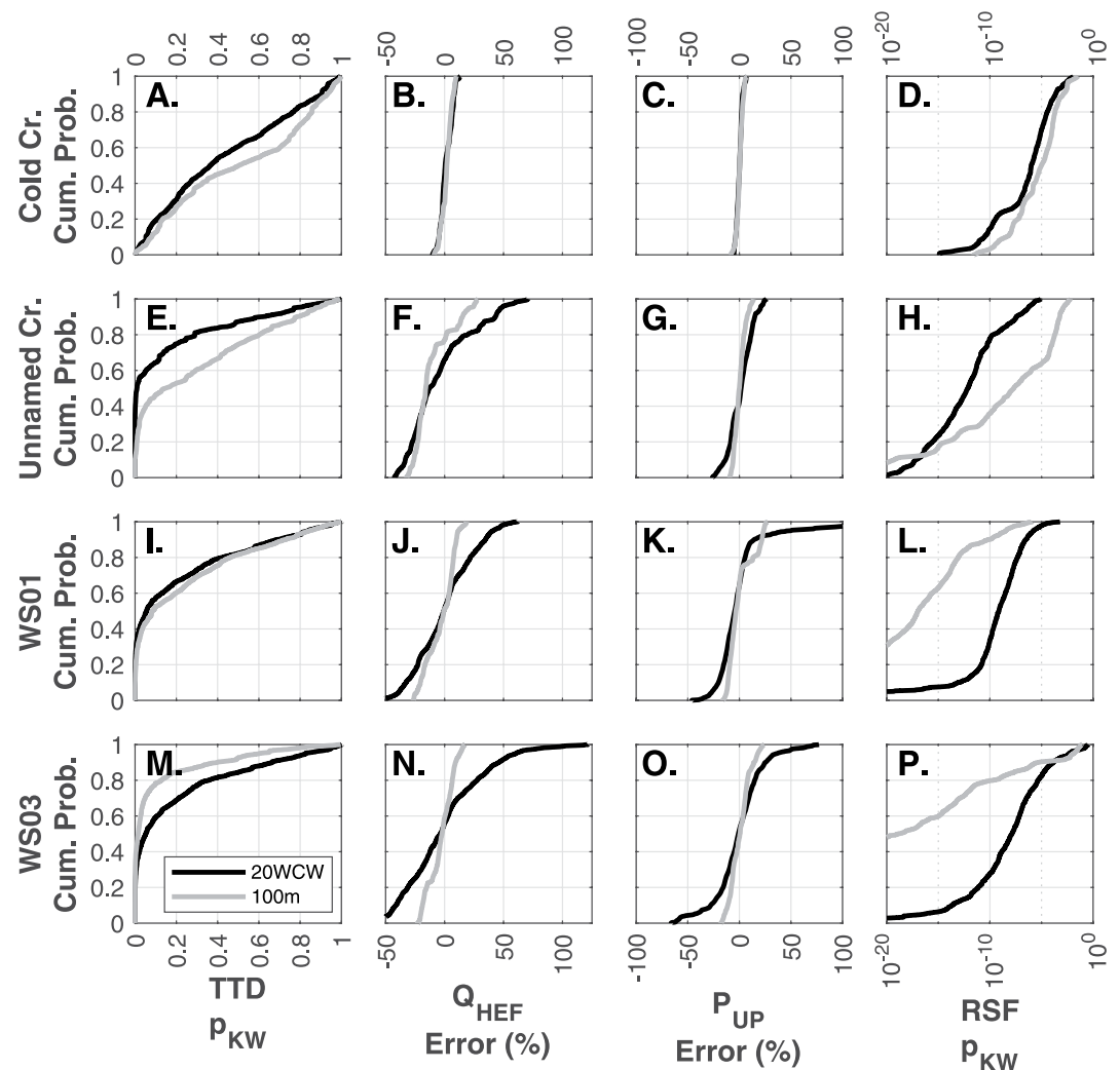
Figure 2. Cumulative distribution functions of both p_{kw} and percent error values for the four metrics: TTD (left column), Q_{hf} (middle-left column), P_{up} (middle-right column), and RSF (right column). Rows from top to bottom are Cold Creek, Unnamed Creek, WS01, and WS03. In all cases, results for 20WCW reaches are shown in solid black, and 100-m reaches are shown in solid gray. For panels (a, d, e, h, i, l, m, and p), a greater portion p_{kw} above 0.10 indicates better representativity compared to the reference reach. For panels (b, c, f, g, j, k, n, and o), a greater portion within \pm 10\% (the narrower the line is), indicates more representativity to the reference reach.
