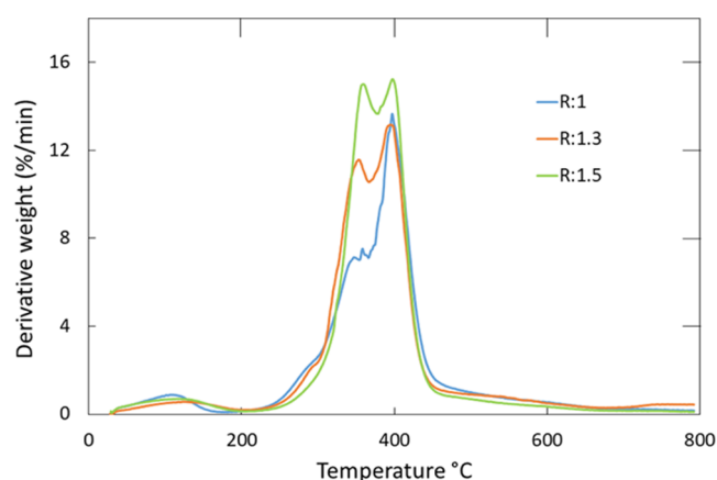
Figure 11. Derivative thermogravimetric analysis (DTG) of OxL-COOH/PEG-epoxy films with different R values.
