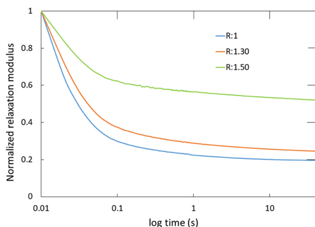
Figure 13. Stress relaxation curves of OxL-COOH/PEG-epoxy films with different R values.
