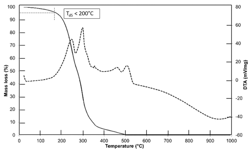
Figure 9. Thermogravimetric analysis (TGA) and derivative thermogravimetric analysis (DTG) study of PEG-epoxy (DTA* in the graph corresponds to DTG analysis). Reprinted with permission from ref 51. Copyright 2020 MDPI. Creative Commons Attribution (CC BY) license ( http://creativecommons.org/licenses/by/4.0/ ).
