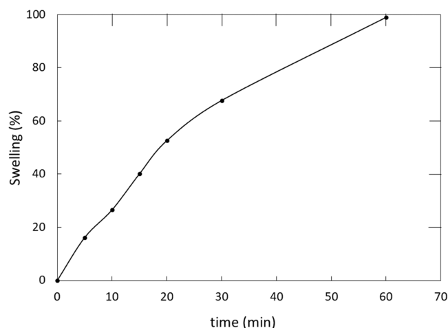
Figure 15. Swelling of OxL-COOH/PEG-epoxy with R:1 in a 0.1 M NaOH solution at different time intervals (0, 5, 10, 15, 20, 30, and 60 min).
