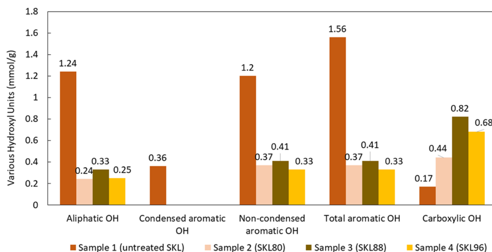
Figure 1. Changes in various hydroxyl units present in softwood kraft lignin before and after oxidation using ^{31}\text{P} NMR.
