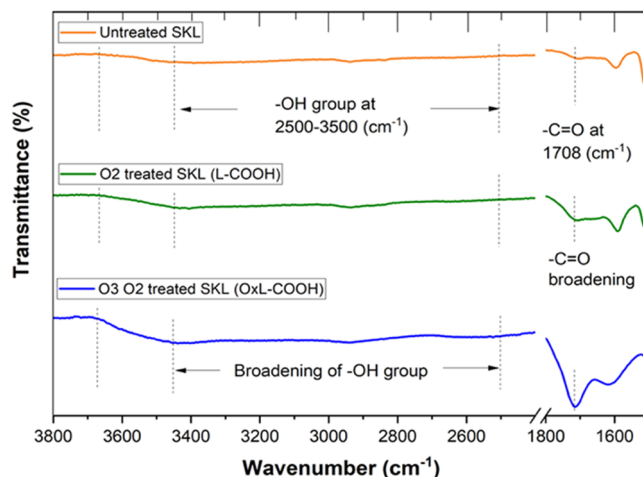
Figure 5. Comparative FTIR spectra of untreated SKL, oxygen-oxidized SKL (L-COOH), and oxygen- and ozone-treated SKL (OxL-COOH). The term O2 represents \text{O}_2 for oxygen oxidation and the term O3 O2 represents sequential oxidation using \text{O}_2 followed by \text{O}_3 oxidation.
