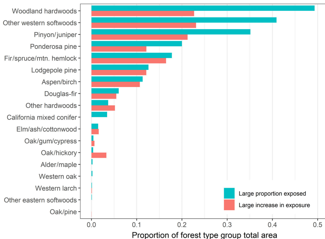
FIGURE 7 Proportion of the total areas of forest type groups that fall within ecological sections where there is high agreement regarding future drought exposure. The top bar in each case represents the proportion of the forest type group's area within ecological sections expected to have greater than average exposure to drought, and the bottom bar represents the proportion of the forest type group's area within ecological sections where the increase in exposure is expected to be greater than average. See Figure 3a,b for where those ecological sections occur. Seven forest type groups analyzed elsewhere in this paper are not listed here because they were entirely outside areas of high agreement.
