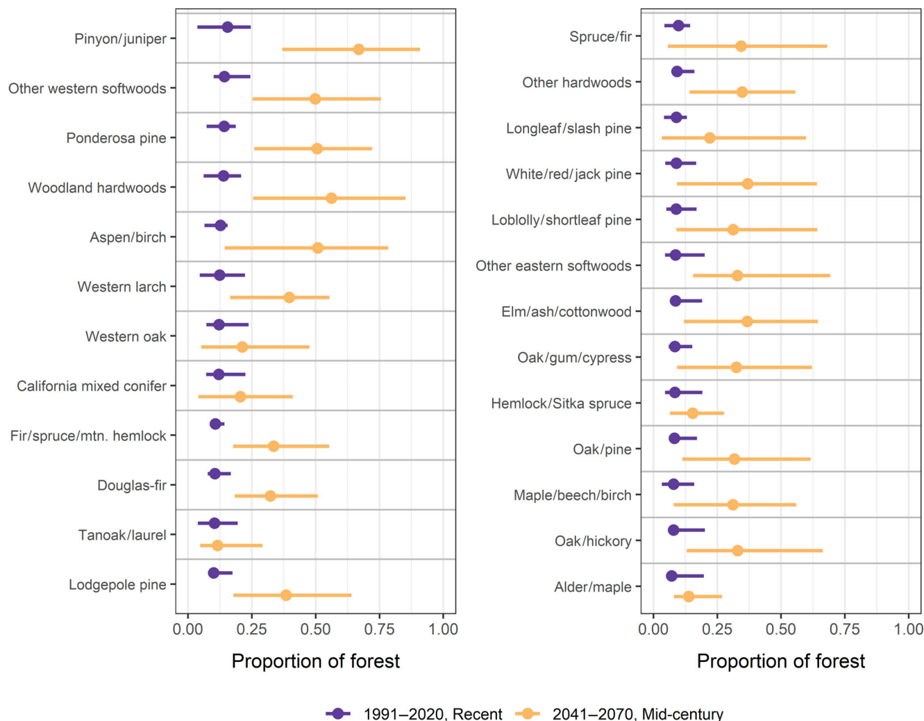
FIGURE 4 Comparison of 30-year average monthly proportion of forest type groups exposed to drought (Standardized Precipitation-Evapotranspiration Index \leq -1.5 ) for the recent and mid-century periods. Dots represent the median of the projections from the 10 scenarios for the given time period, and horizontal bars indicate the range of values across those projections. Forest type groups are listed here in decreasing order of median proportion exposed in the recent period.
