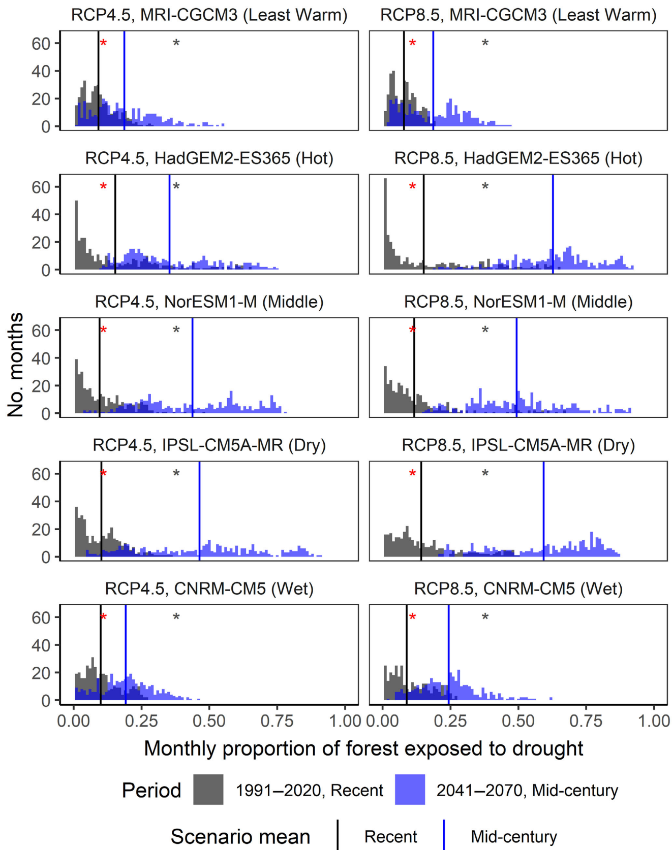
FIGURE 1 Histograms of proportion of US forest exposed to drought (Standardized Precipitation-Evapotranspiration Index \leq -1.5 ) in the recent and mid-century time periods. Solid lines indicate mean proportion for each time period for individual scenarios. Red and gray asterisks indicate overall means across the 10 scenarios for the recent and mid-century time periods, respectively, and do not change across the panels. RCP, Representative Concentration Pathway.
