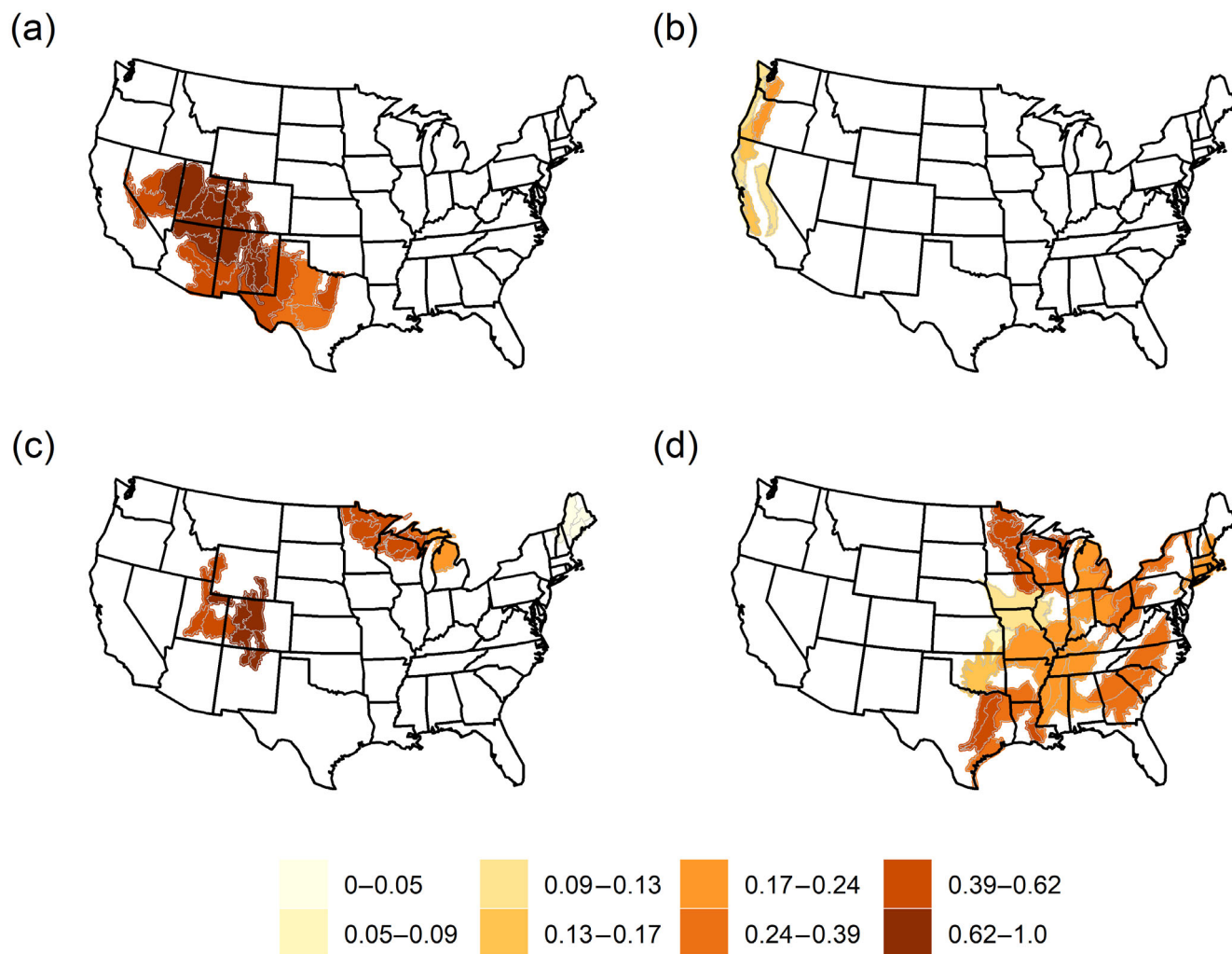
FIGURE 5 Proportion of forest type group's area within each ecological section that was projected to be exposed to drought (Standardized Precipitation-Evapotranspiration Index \leq -1.5 ) in the HadGEM2-ES365, Representative Concentration Pathway 4.5 scenario for the mid-century period. This scenario had exposure values that were closest to the overall mean for the mid-century period. Maps show (a) pinyon/juniper, (b) tanoak/laurel, (c) aspen/birch, and (d) maple/beech/birch forest type groups. Ecological sections that are less than 10% forested as well as those that contain less than 1% of the forest type group's area were included in analyses but are not shown on the maps. Classes displayed here are the same as in Figure 2 and were determined by quantile (equal frequency) classification across all forest type groups and scenarios. See Appendix S2 for maps of all forest type groups under each of the 10 scenarios.
