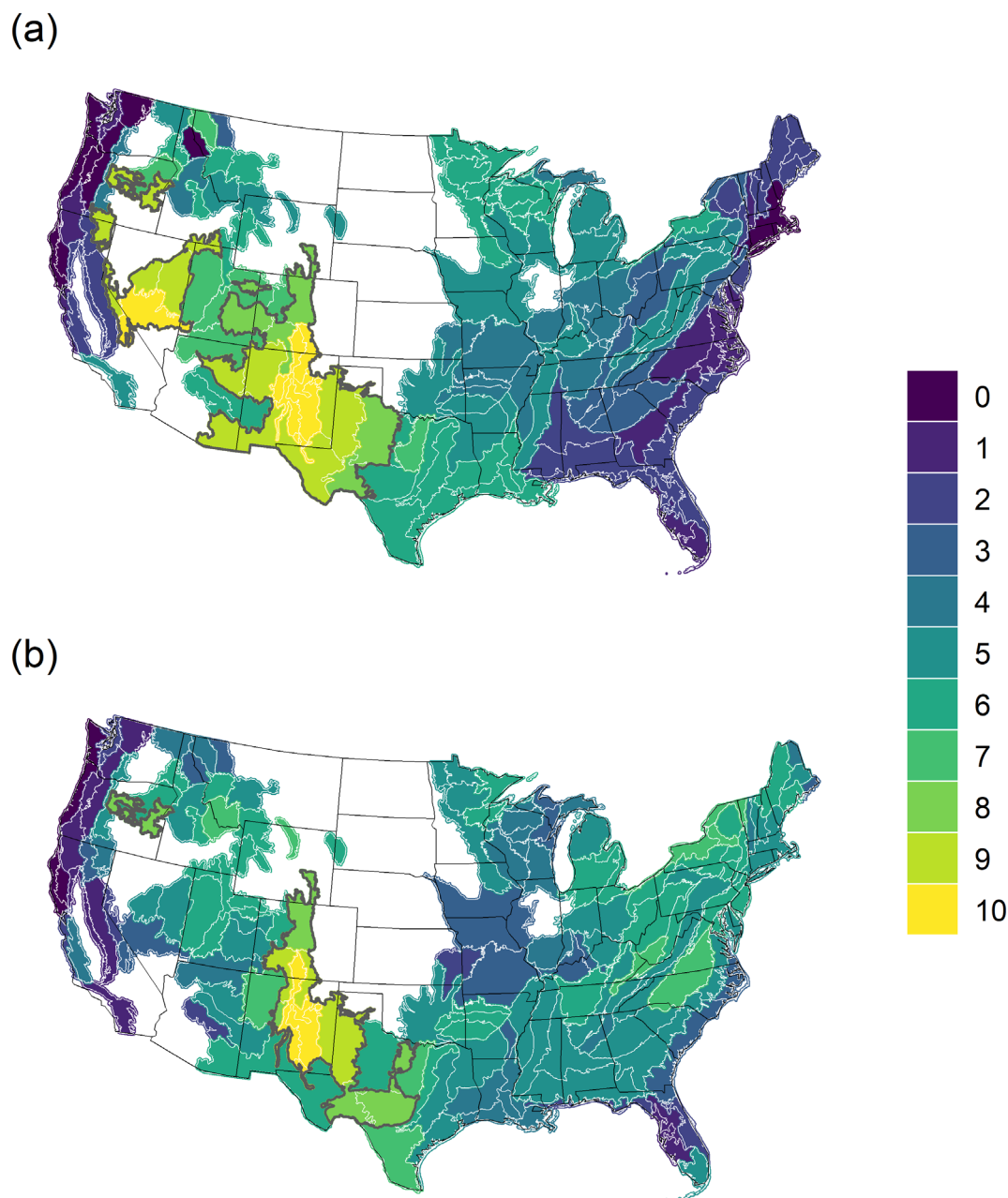
FIGURE 3 Number of scenarios projecting (a) greater than the US average of 37.8% of forest exposed to drought for mid-century and (b) greater than the US average of 238% increase in proportion of forest exposed to drought. Ecological sections that are less than 10% forested are not shown. Ecological sections labeled 8, 9, or 10 on each of these maps were considered places of high agreement and are outlined in black.
