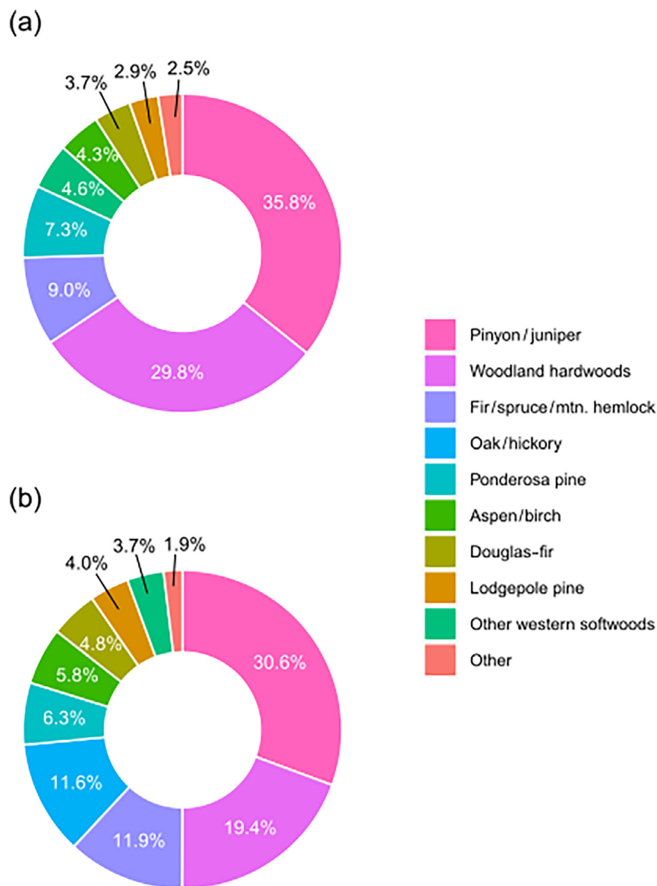
FIGURE 6 Composition of forest type groups in areas of high agreement among the modeled scenarios that (a) the average monthly proportion of forest exposed at mid-century will be greater than the overall average, and (b) the increase in average monthly exposure by mid-century will be greater than the overall average. Areas of high agreement are ecological sections where projections for at least 8 of the 10 scenarios are indicated in Figure 3a,b. Forest type groups that made up at least 1.5% of the forest in high-agreement areas are listed. The “other” category in both panels is composed of forest type groups that individually made up less than 1.5% of the forest.
