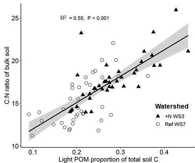
Fig. 3. Significant and positive relationship between the proportion of total soil C in the light particulate organic matter (POM) fraction and the C:N ratio of bulk soil from the reference watershed (Ref WS7, open circles) and fertilized watershed (+N WS3, black triangles). Black line represents the linear regression with standard error (gray shading).
