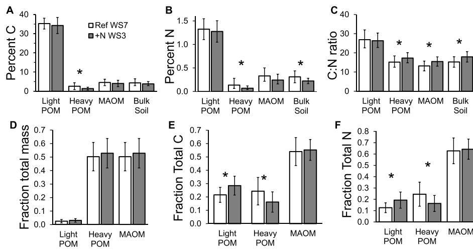
Fig. 2. Soil density fractionation results for the reference watershed (Ref WS7, white bars) and fertilized watershed (+N WS3, gray bars). Mean ( \pm se) of the percent C (A), percent N (B), and C:N ratio (C) of light particulate organic matter (POM), heavy POM, mineral-associated organic matter (MAOM) and bulk soil. The mean ( \pm se) fraction of total bulk soil mass (D), carbon (E), and nitrogen (F) for the three soil fractions. Asterisks denote significant difference between watersheds (ANOVA, P < 0.05 ).
