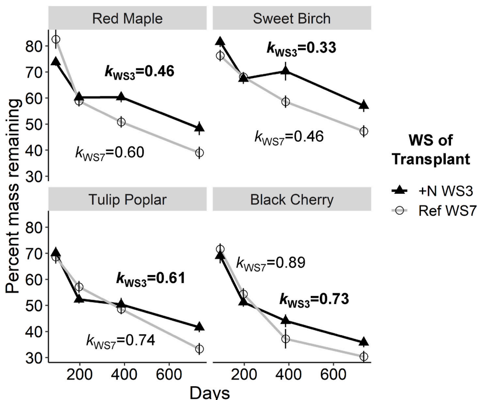
Fig. 1. Percent of initial leaf litter mass remaining over two-year litter decomposition in the field for four dominant tree species. Mean \pm se of percent mass remaining for litter transplanted into the fertilized watershed (+N WS3; black triangles) and reference watershed (Ref WS7; open circles). Decomposition rates ( k ) displayed for each watershed and species combination. Decomposition rates ( k ) differed between watershed of transplant for all species, and there was no effect of watershed of litter origin on decomposition rates (but see Fig. S2).
