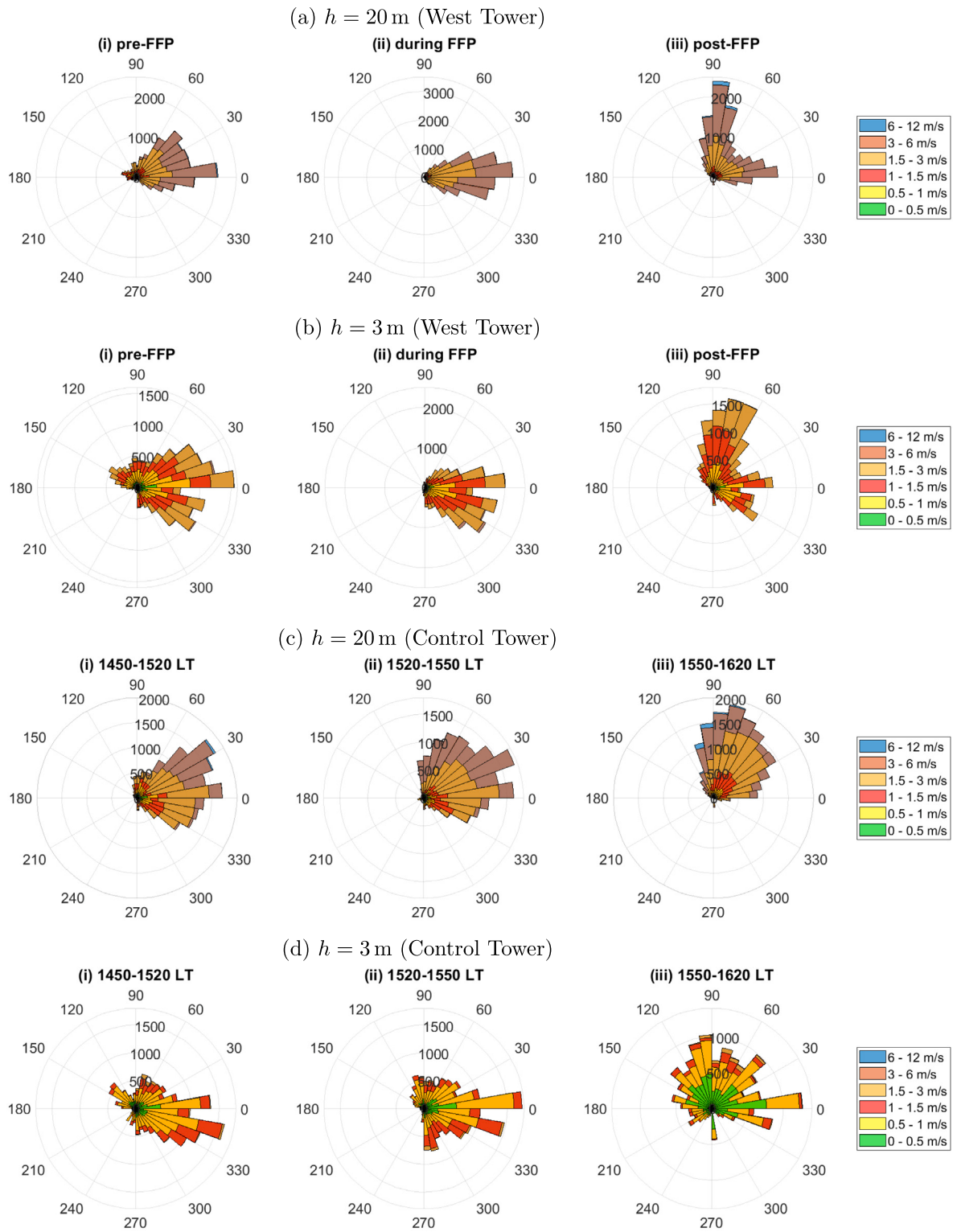
Fig. 3. Total horizontal velocity ( \hat{u} + \hat{v} ) wind-rose statistics for (i) pre-FFP, (ii) FFP, and (iii) post-FFP times at (a) h = 20 m and (b) h = 3 m at the West Tower for NJ2019, and at (c) h = 20 m and (d) h = 3 m, during the each of those durations, at the Control Tower for NJ2019. Colors represent classes of wind speed, while 0° represents the positive streamwise direction.
