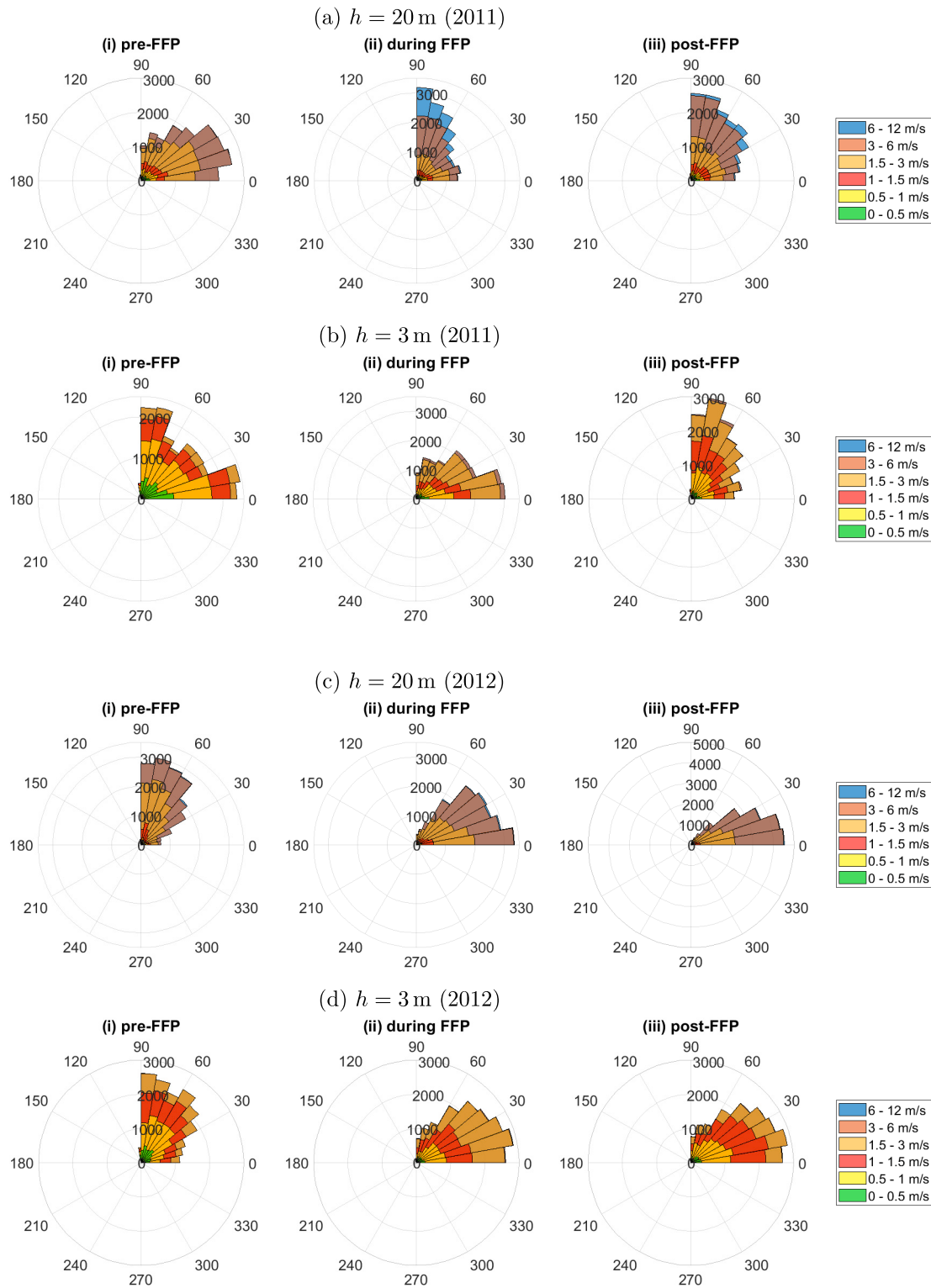
Fig. 2. Total horizontal velocity ( \hat{u}\hat{i} + \hat{v}\hat{j} ) wind-rose statistics for (i) pre-FFP, (ii) FFP, and (iii) post-FFP times at (a) h = 20 m and (b) h = 3 m for NJ2011, and for (c) h = 20 m and (d) h = 3 m for NJ2012. Colors represent classes of wind speed, while 0^\circ represents the positive streamwise direction.
