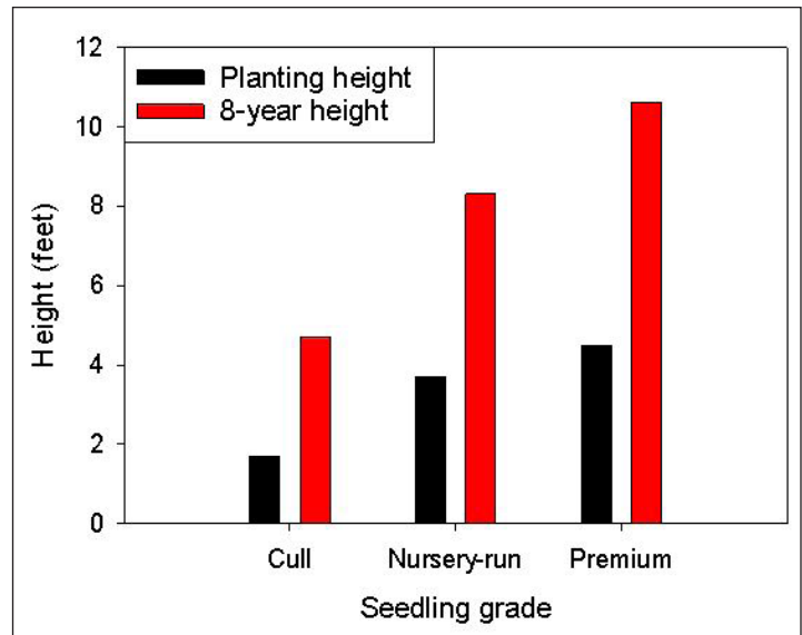
Figure 4: Increased mean growth from seedling grading after 8 years for northern red oak seedlings planted in a commercial clearcut in southwestern North Carolina (Clark, unpublished data).
