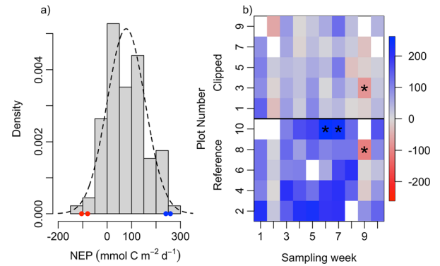
Figure 4. Seagrass metabolism (NEP, \text{mmol C m}^{-2} \text{d}^{-1} ) in ten experimental plots across ten sampling weeks. a Histogram of empirical values overlain by a reference Gaussian distribution with equal mean and variance to the empirical distribution. Extreme negative and positive values are identified, respectively, by red and blue points. b NEP values across plots and sampling weeks. Extremes are indicated with an asterisk. White cells are times when metabolism measurements are missing for a given plot. The fact that no plots or sampling weeks predominate the set of extreme observations supports the conclusion from the test for HSHM presence that this case study does not reflect HSHM.
