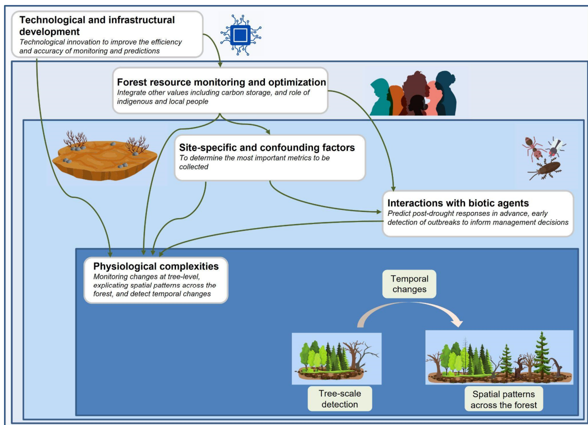
Figure 2. Conceptual framework for the prospective approaches and recommendations for using UAV-based technologies to monitor drought impacts at different scales, early detection of post-drought outbreaks, and how to integrate site-specific, confounding factors and other values in developing the early warning metrics. Also shown are technological innovations that could, in general, improve the efficiency and accuracy of monitoring and prediction of drought impacts.
