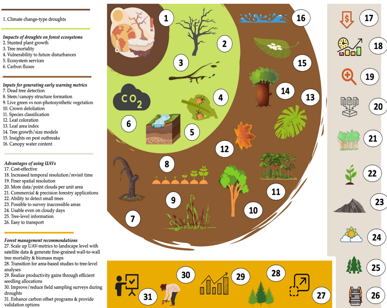
Figure 1. Impacts of climate-change-driven droughts on forests and possible pathways through which operationalization of UAV-derived early warning indicators can assist post-drought tree mortality and biomass assessment.
