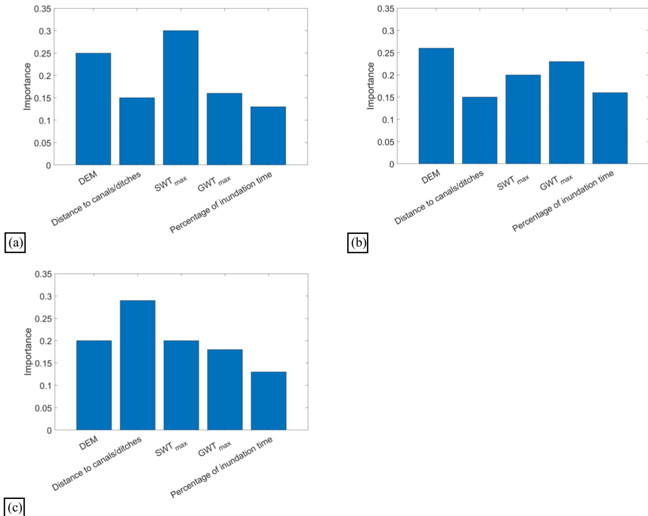
Fig. 4. The variable importance analysis in the three random forest (RF) models. (a) RF1: DW and NDW, (b) RF2: DH and NDH, and (c) RF3: W2N and W2H. DEM represents the digital elevation model. SWT_{max} and GWT_{max} stand for the maximum seasonal saltwater and groundwater tables, respectively.
