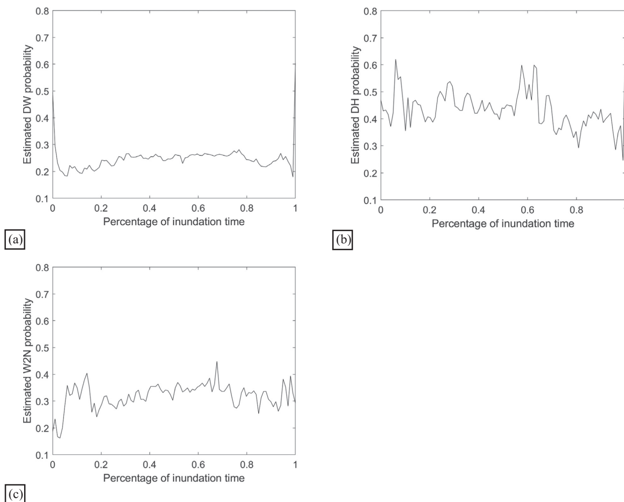
Fig. 7. Partial dependence plot of the variable PIT for (a) DW and NDW, (b) DH and NDH, and (c) W2N and W2H.
