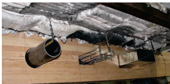
Figure 3: Glulam beam (Type C) with penetrations for a pipe, cable tray and duct (left to right).
