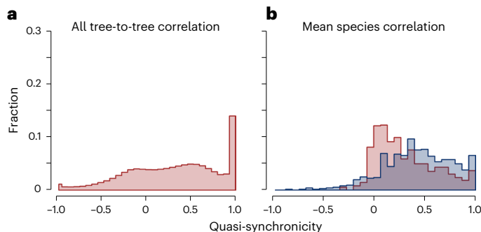
Fig. 4 | Quasi-synchronicity at individual and species level. a. Correlations between every pair of trees of the same species within 1 km show a mode near one, but a broad range. b. Species average correlations are concentrated near zero (red), but fecundity-weighted correlations are substantially higher (blue) (Methods).
