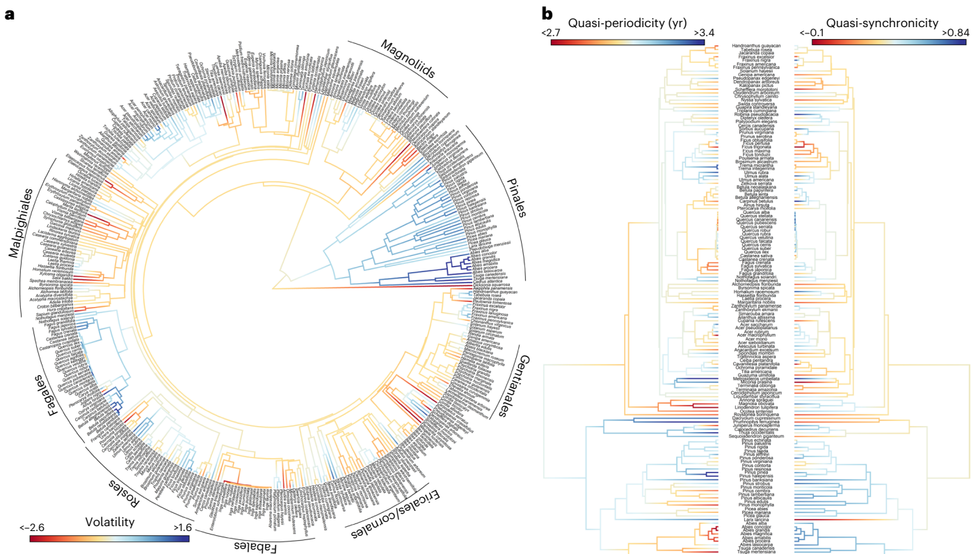
Fig. 6 | Phylogenetic coherence in the three masting components. a , Volatility (on log scale) has a phylogeny component (Pagel's \lambda = 0.83 , P < 10^{-9} , n = 394 ). b , Quasi-periodicity (left) exhibits a weaker phylogenetic coherence compared with volatility (Pagel's \lambda = 0.52 , P = 0.0023 , n = 142 ). Quasi-synchronicity (right)
