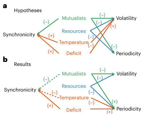
Fig. 2 | Hypothesized effects and summary of results in this study. a, b, We summarized the results ( b ) after testing the hypotheses ( a ) related to the effects of mutualists (green), resources (blue), and climate (red) on the three masting components. Arrows with (+) and (-) represent positive and negative effects, respectively. We expect that tree species with low volatility, short periodicity and low synchronicity benefit most from their mutualist pollinators and dispersers ( a ). Resources reduce volatility and periodicity ( a ). High temperature decreases volatility while promoting synchronicity ( a ). Dry sites (deficit) have higher volatility and synchronicity than wet sites ( a ). The summary of results in b comes from the joint model in Fig. 3. Dashed lines indicate that 90% credible intervals contain zero while 68% credible intervals do not.
