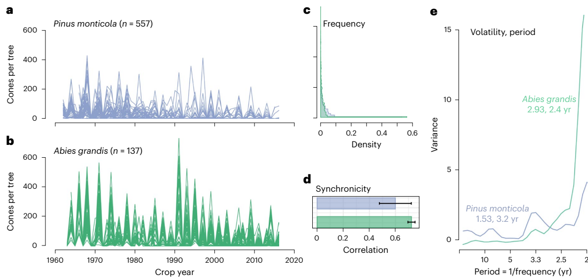
Fig. 1 | Illustration of three masting components for representative tree species from the central Cascades, USA. a, b, Crop counts for P. monticola and A. grandis vary between individual trees and drift over time. c, The frequency of counts in both species shows that zeros dominate, and there is no threshold that could be used to define masting events. d, Mean pairwise correlations between
