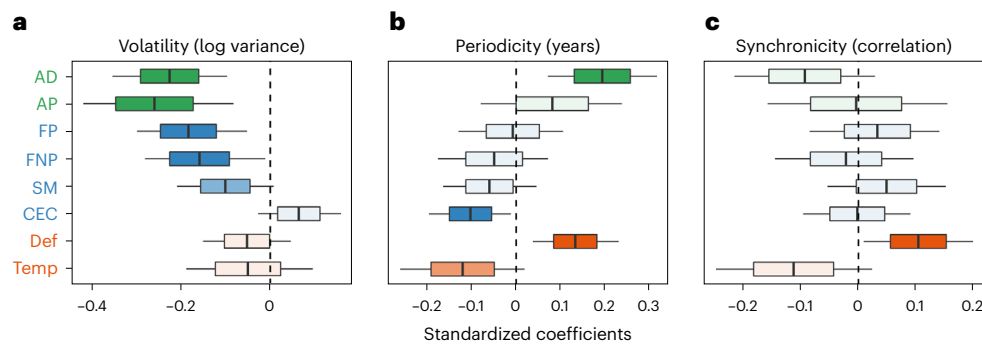
Fig. 3 | The joint response of mast components to mutualist dispersers, resources and climate. a–c. Three mast components include volatility (a), periodicity (b) and synchronicity (c) at ecoregion–species scales. Predictors include vertebrate dispersers (animal seed dispersal (AD) and animal pollination (AP)), resources (soil cation exchange capacity (CEC), foliar P (FP) and foliar N:P ratio (FNP)), seed mass (SM) and climate (accumulated moisture deficit (Def, ranging from wet to dry) and mean annual temperature (Temp, ranging from cold to warm)). Dispersal and pollination syndromes are included as two-level factors, so the negative coefficients for AD and AP have as mirror images the positive
