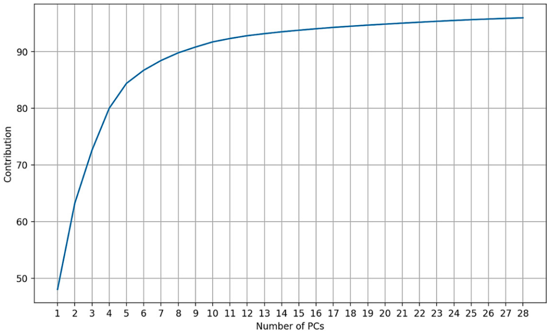
Figure 6. Contribution of PCs to the data.
