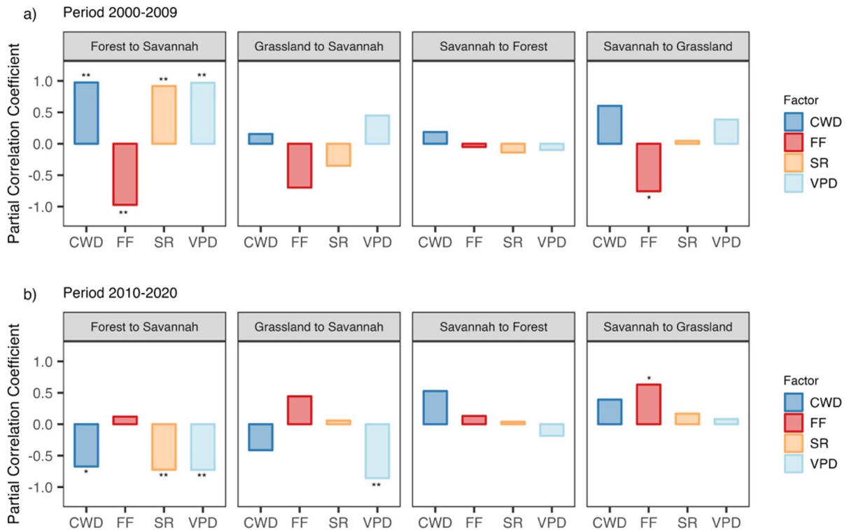
Fig. 7 Partial correlation coefficients between the tree cover and the environmental factors: climatic water deficit (CWD), fire frequency (FF), vapor pressure deficit (VPD), and downward surface shortwave radiation (SR). Subfigures (a) and (b) show partial correlation coefficients for the environmental factors in four types of land conversions during the periods 2000–
