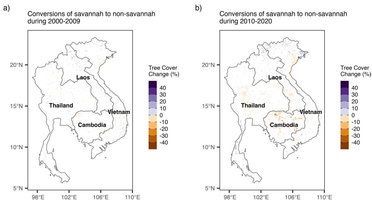
Fig. 6 Spatial distributions of savannahs converting to forests or grasslands and associated tree cover changes in mainland Southeast Asia (MSEA) during the earlier (a) and latter (b) periods. The earlier period was from 2000 to 2009 and the latter from 2010 to 2020
