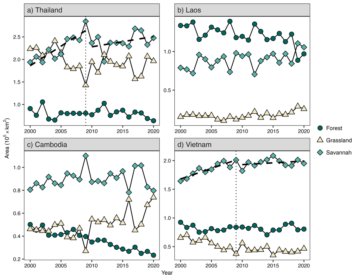
Fig. 3 Annual area of forest, savannah, and grassland during 2000–2020 in four countries of mainland Southeast Asia (MSEA): Thailand ( a ), Laos ( b ), Cambodia ( c ), and Vietnam ( d ). Forest is indicated as dark green and circle points. Savannah is indicated as light green and diamond points. Grassland
