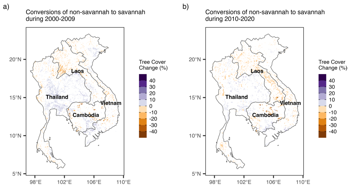
Fig. 5 Spatial distributions of forests and grasslands converting to savannahs and associated tree cover changes in mainland Southeast Asia (MSEA) during the earlier (a) and latter (b)
