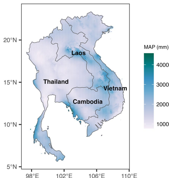
Fig. 1 The study is focused on four countries of mainland Southeast Asia (MSEA): Thailand, Laos, Cambodia, and Vietnam. The filling values indicate mean annual precipitation (MAP)
