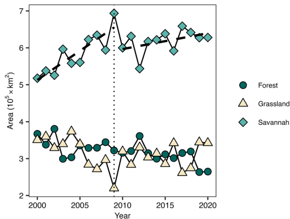
Fig. 2 Annual areas of forest, savannah, and grassland during 2000–2020 in mainland Southeast Asia (MSEA). Forest is indicated as dark green and circle points. Savannah is indicated as light green and diamond points. Grassland is indicated as yellow and triangle points. The vertical dotted line indicates the year (2009) where the breakpoint for the savannah area change is detected. The segmented dashed lines are the linear trend lines before and after the breakpoint
