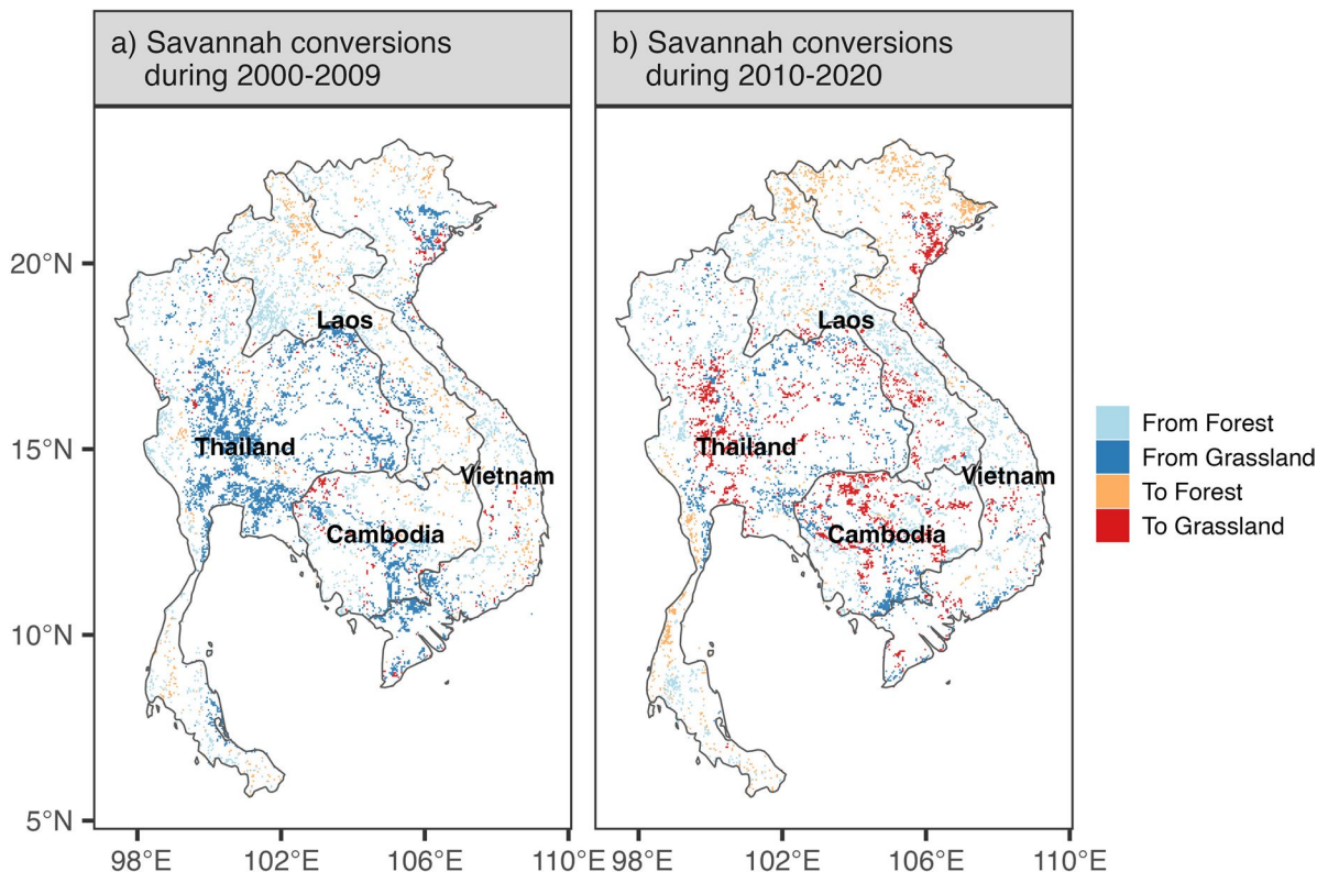
Fig. 4 Conversions between savannahs and other land cover types across mainland Southeast Asia (MSEA) during 2000–2009(a) and 2010–2020 (b). The savannah-related conversions
