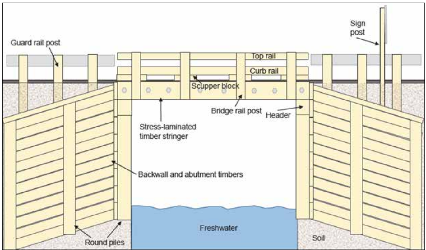
FIGURE 1. Critically important wood components supporting timber bridges (Lebow et al., 2019).
