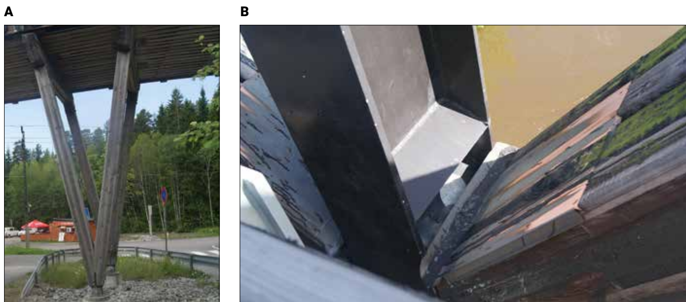
FIGURE 5. V-shaped joint (a) and cladding of an inclined frame (b) to promote water escaping (Massaro and Malo, 2014).
