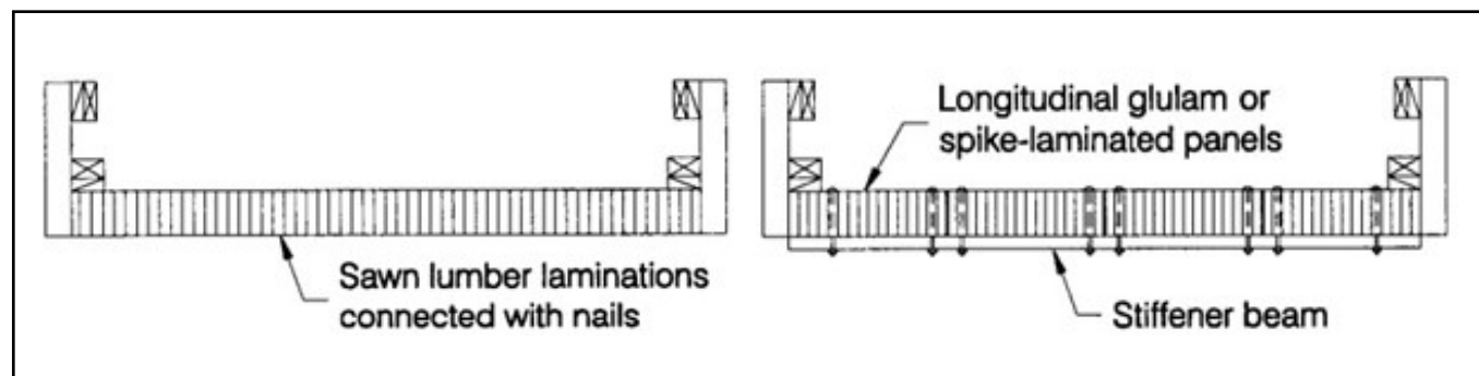
FIGURE 2. Typical configuration of the end view of a nail laminated deck system and a longitudinal glulam or spike-laminated panel deck system. (Summary only, full details in Wacker and Smith, 2001).
