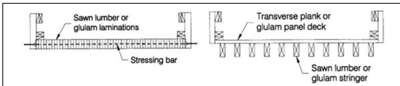
FIGURE 3. End view of stress-laminated deck system and longitudinal stringer bridge (Lee et al., 1995).
