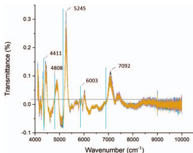
Figure 4.—Second derivative of the transmittance of the downed pine trees.
