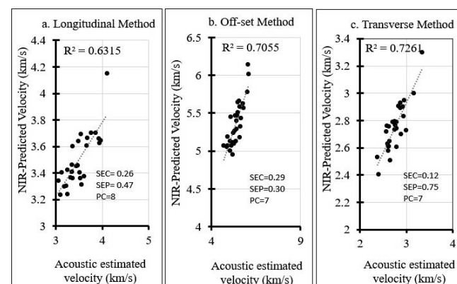
Figure 5.—Relationship between measured acoustic velocity and NIR-fitted velocity.
