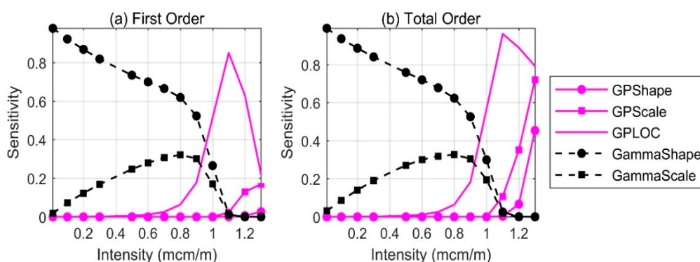
Figure 2. (a) The first order and (b) the total order sensitivity indices of Mixture Gamma-GPD model for drought return period.
