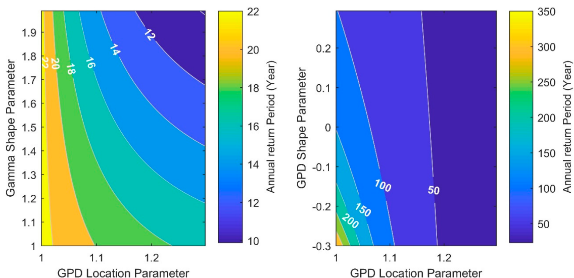
Figure 3. Sensitivity of drought return period to Gamma shape parameter and GPD location parameter below the threshold ( left-panel ) and GPD shape and GPD location parameters over the threshold ( right-panel ).
