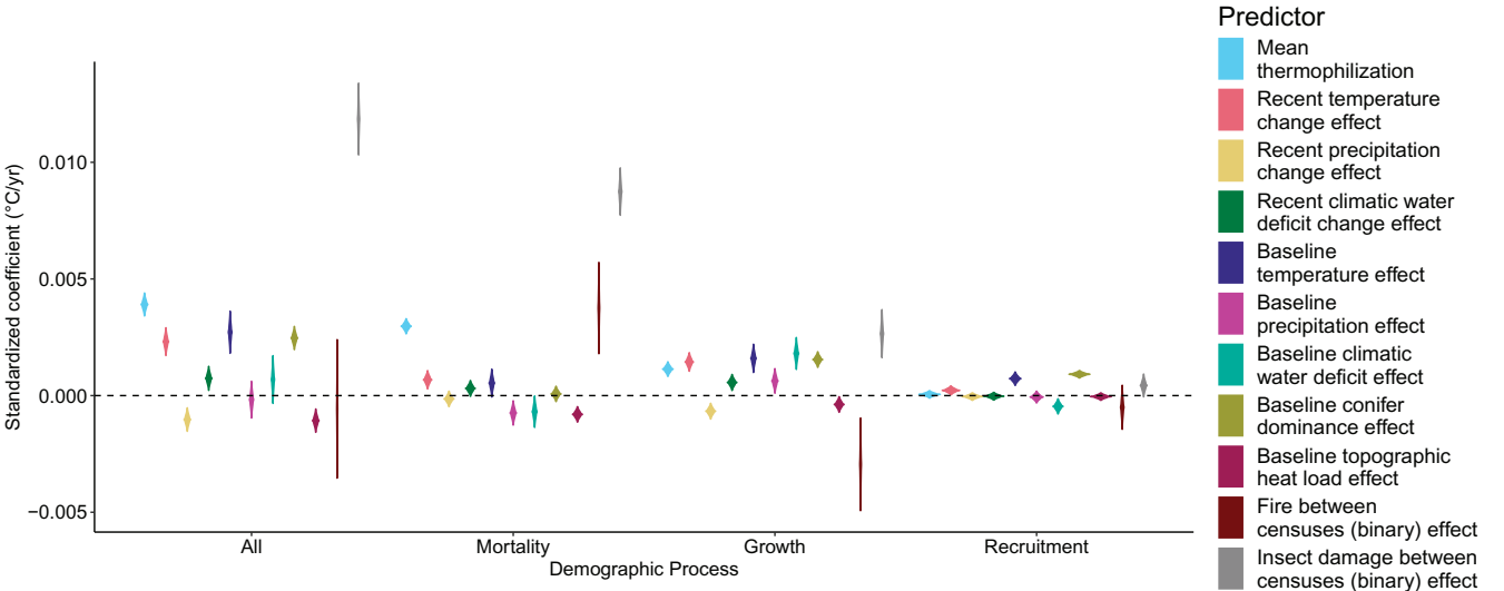
Fig. 4. Violin plots of 95% credible intervals for standardized effects of fixed predictors on the magnitude of thermophilization in western US tree communities. Results come from hierarchical Bayesian regression models of tree community temperature index over time. Violins can be interpreted as smoothed, horizontally symmetrical histograms, with the vertical axis representing parameter values and the horizontal axis representing probability density. The total area of each violin is set to be equal, so shorter and wider violins correspond to model parameters for which the posterior probability density is more concentrated around the mean. The interval for mean thermophilization represents the effect size for a binary “T1 vs. T2” predictor that distinguishes between repeat tree censuses. The interval shown for each other predictor represents the effect size for the interaction between the named predictor and the “T1 vs. T2” predictor.
