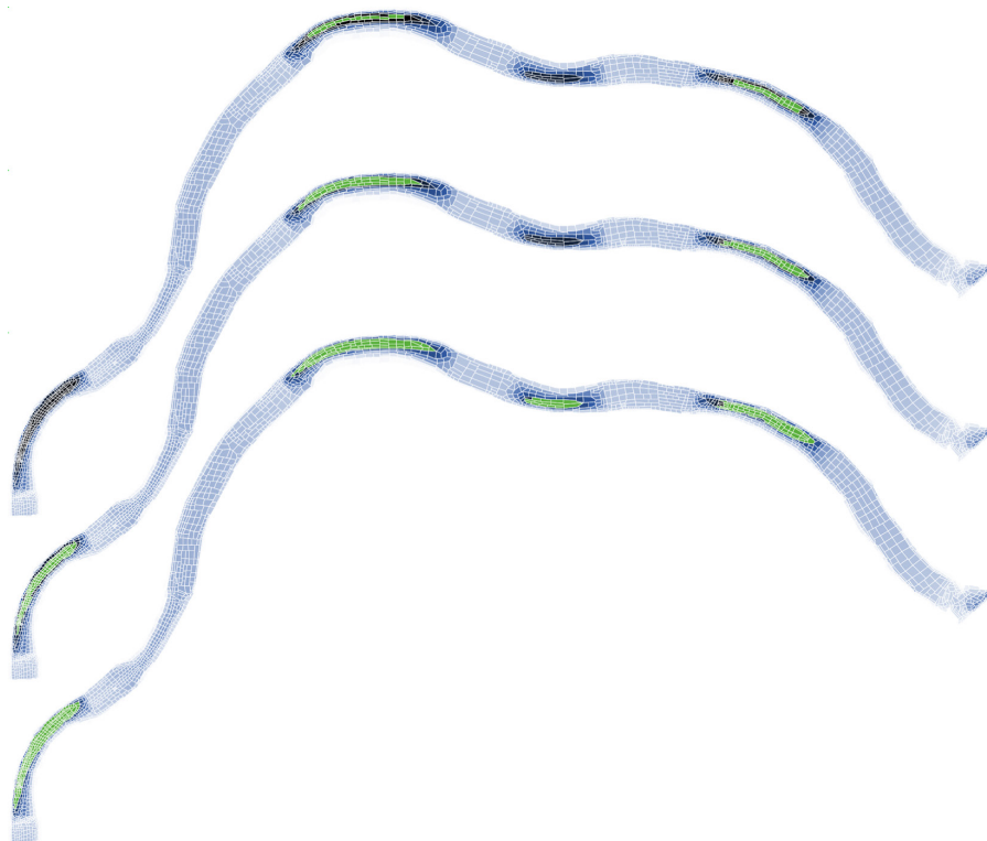
FIGURE 1 The simulated stream reach under (top to bottom) low, medium, and high refuge availability. Cells are shaded by depth, with darker being deeper; cells providing thermal refuge at a flow of 4.0 \text{ m}^3/\text{s} are green.
