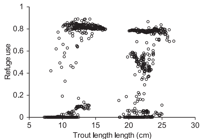
FIGURE 3 Refuge use by individual simulated fish; each point represents one fish, indicating (y-axis) the percentage of time steps it spent in refuges over the May–August simulation period versus (x-axis) its mean length during the simulation. Fish <16 cm are age 1, and fish >16 cm are age 2. Results include fish that died during the simulation.
