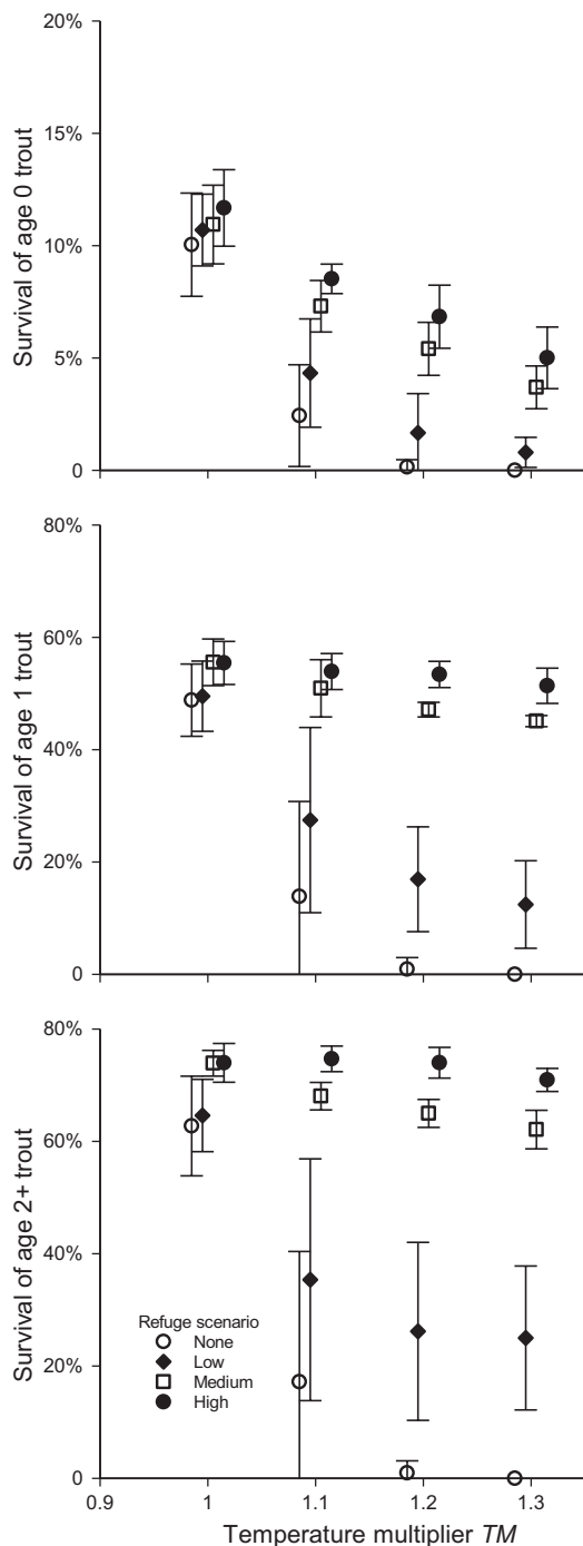
FIGURE 5 Survival results for (top to bottom) ages 0, 1, and 2+. Symbols and error bars indicate the mean and standard deviation, respectively, over the five simulated years. Points are offset around the temperature multiplier ( TM ) values to increase clarity.
