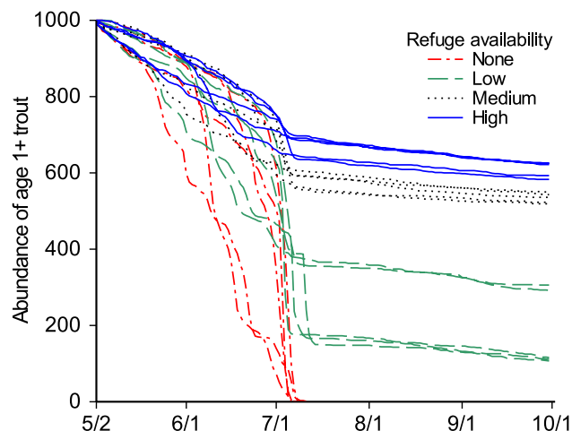
FIGURE 6 Time series of age-1+ salmonid abundance over May–September for the four refuge availability scenarios and warmest temperature scenario ( TM=1.3 ). Separate lines represent the 5 years simulated for each refuge scenario.
