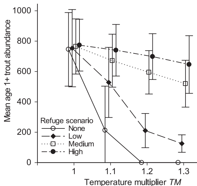
FIGURE 12 Response of long-term mean salmonid abundance to temperature regime and refuge availability. The y-axis is the mean of adult abundance on September 30 over simulated years 2003–2022. Error bars represent standard deviation over the 20 annual values of five replicate simulations.
