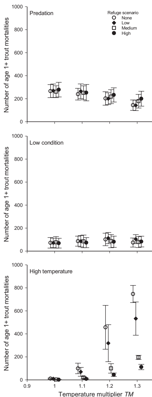
FIGURE 7 Causes of mortality: number of simulated salmonids age 1 and older dying of predation, poor condition (disease and starvation), and acute temperature stress. Format is as in Figure 5 except that ages 1 and 2+ are combined as adults (age 1+).
