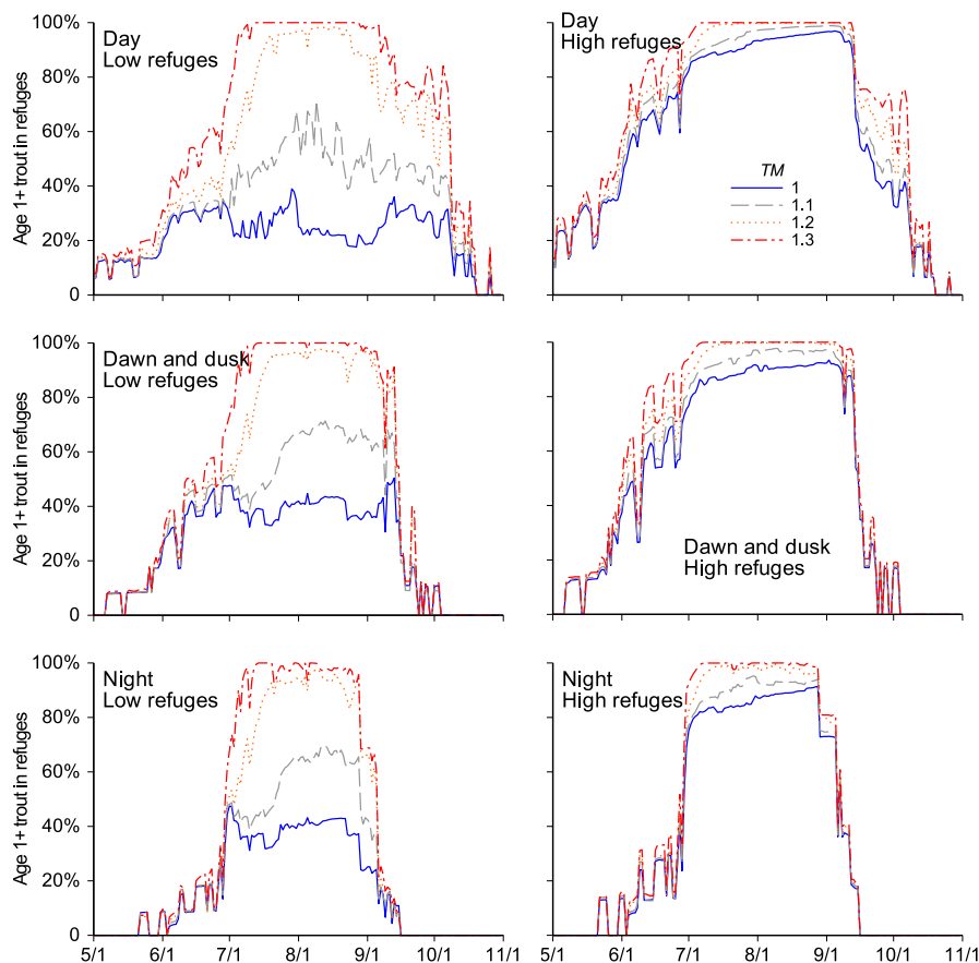
FIGURE 9 Refuge use: percentage of salmonids age 1 and older occupying refuge pools in low (left panels) and high (right panels) refuge availability scenarios during the three daily light conditions. Combined results over all five simulated years.
