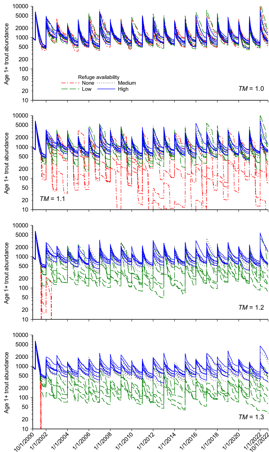
FIGURE 11 Long-term simulation results. Each line represents the results of one of five simulations for each refuge scenario. From top to bottom, panels report results for the TM from 1.0 to 1.3.
