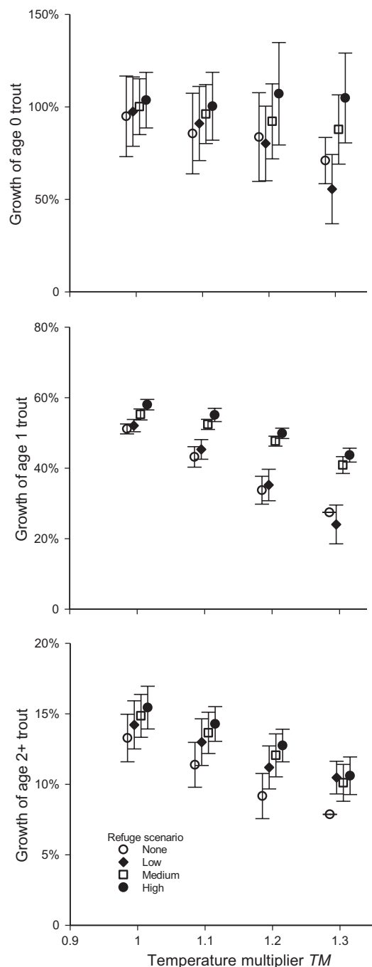
FIGURE 8 Simulated March–October growth. Format as in Figure 5.
