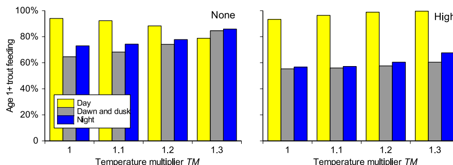
FIGURE 10 Example effect of refuges on when salmonids feed, with no (left panel) and high (right panel) refuge availability. Bars indicate the mean percentage of age-1+ fish feeding by time of day in July–September of five simulated years.
