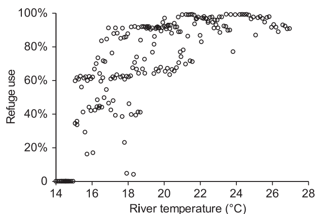
FIGURE 2 Simulated refuge use versus river temperature, May–August 2002, with a temperature multiplier of 1.1. Each point represents one time step; the x-axis is the temperature outside thermal refuges, and the y-axis is the percentage of adult (age 1 and older) salmonids in a refuge.
