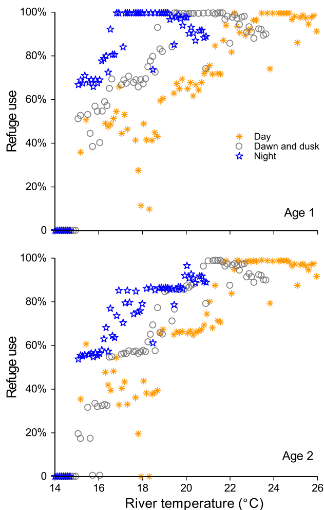
FIGURE 4 Refuge use versus river temperature, categorized by fish age and time of day.
