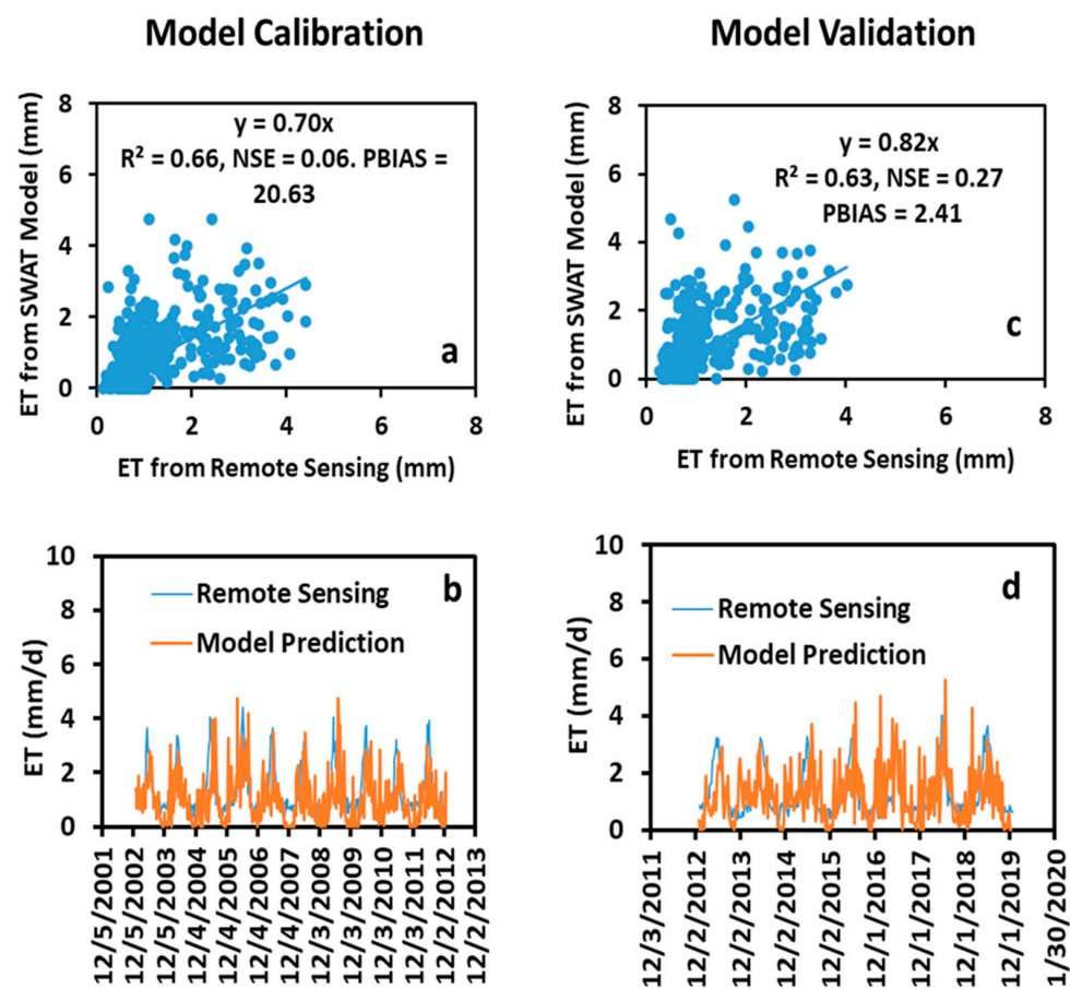
Figure 3. Comparisons of the MODIS-measured and SWAT-predicted daily ETs during the model calibration (a,b) and validation (c,d).
