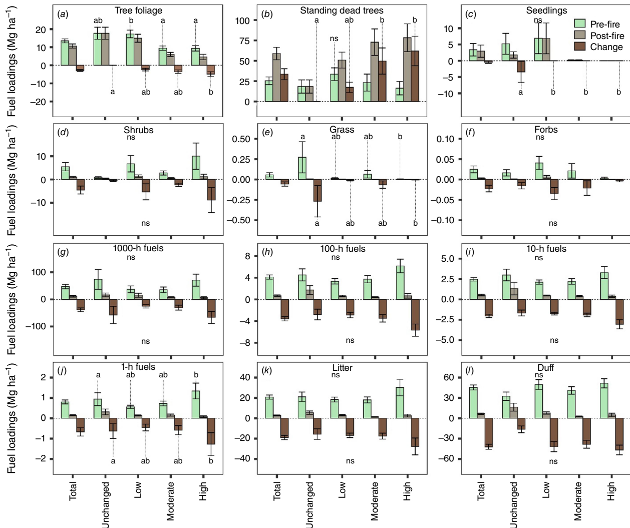
Fig. 3. The pre- and post-fire fuel loadings ( \text{Mg ha}^{-1} ) by fuel strata for 112 mixed-conifer forests in California, USA. Error bars are \pm 1 standard error. Biomass is plotted for pre-, post-fire and the change in biomass for (a) live overstorey foliage biomass, (b) standing dead tree bole fuels, (c) seedling fuels, (d) shrub fuels, (e) grass fuels, (f) forb fuels, (g) 1000-h fuel fuels, (h) 100-h fuel fuels, (i) 10-h fuel fuels, (j) 1-h fuels, (k) litter fuels, and (l) duff fuels. Lowercase letters indicate significant differences in pre-fire biomass and post-fire change ( P < 0.05 ) among severity categories. Non-significant differences are denoted by 'ns'.
