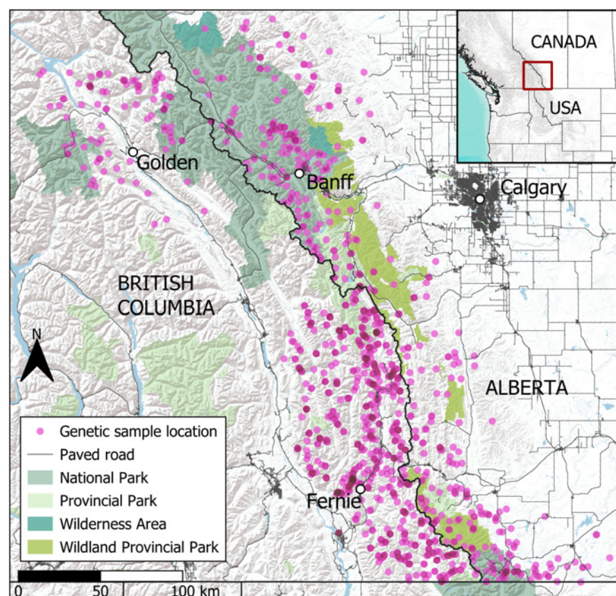
FIGURE 1 Study area and locations of 1161 grizzly bear genetic samples in south-east British Columbia and south-west Alberta, Canada. Darker colours indicate overlapping sample locations. [Colour figure can be viewed at wileyonlinelibrary.com ]
