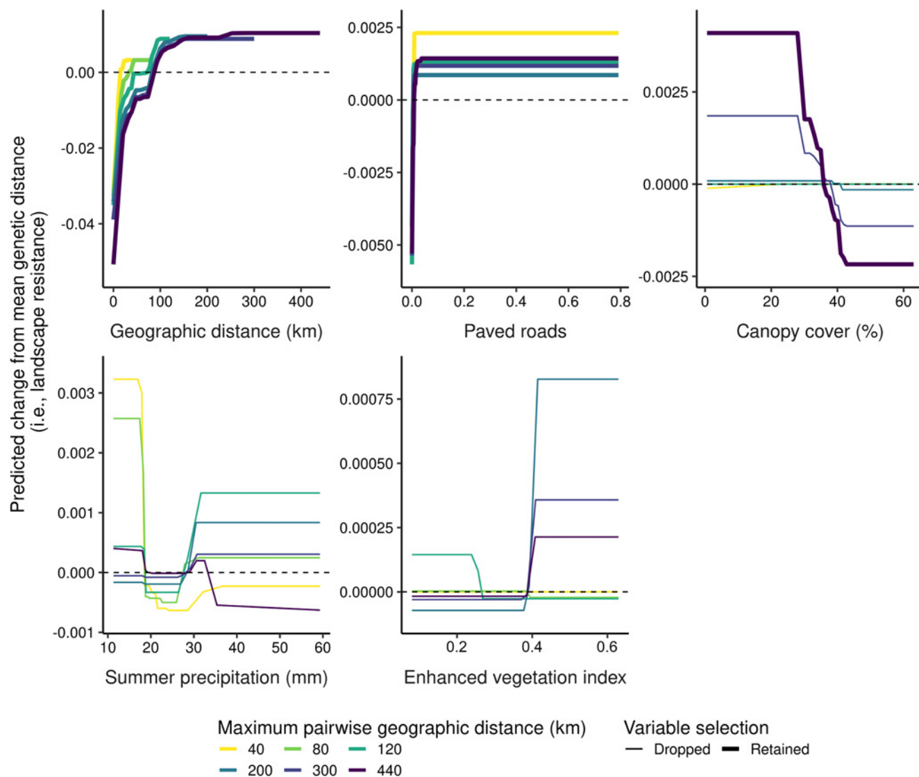
FIGURE 3 Accumulated local effect plots showing the predicted change in genetic distance from GBMs at six different spatial scales using data from 1161 grizzly bears ( Ursus arctos ) in Canada's southern Rocky Mountains across a range of values for different landscape variables. Values on the y-axis depict the main effect of the variable at a certain value compared to the average predicted genetic distance (which is 0) between all pairwise combinations of bears in the entire dataset. Therefore, positive y-axis values indicate higher predicted genetic distance than average or more landscape resistance. Note that the y-axis differs across panels. Terrain ruggedness and glaciers were not included because they were rarely influential and their effects across spatial scales produced no discernible pattern. [Colour figure can be viewed at wileyonlinelibrary.com ]
