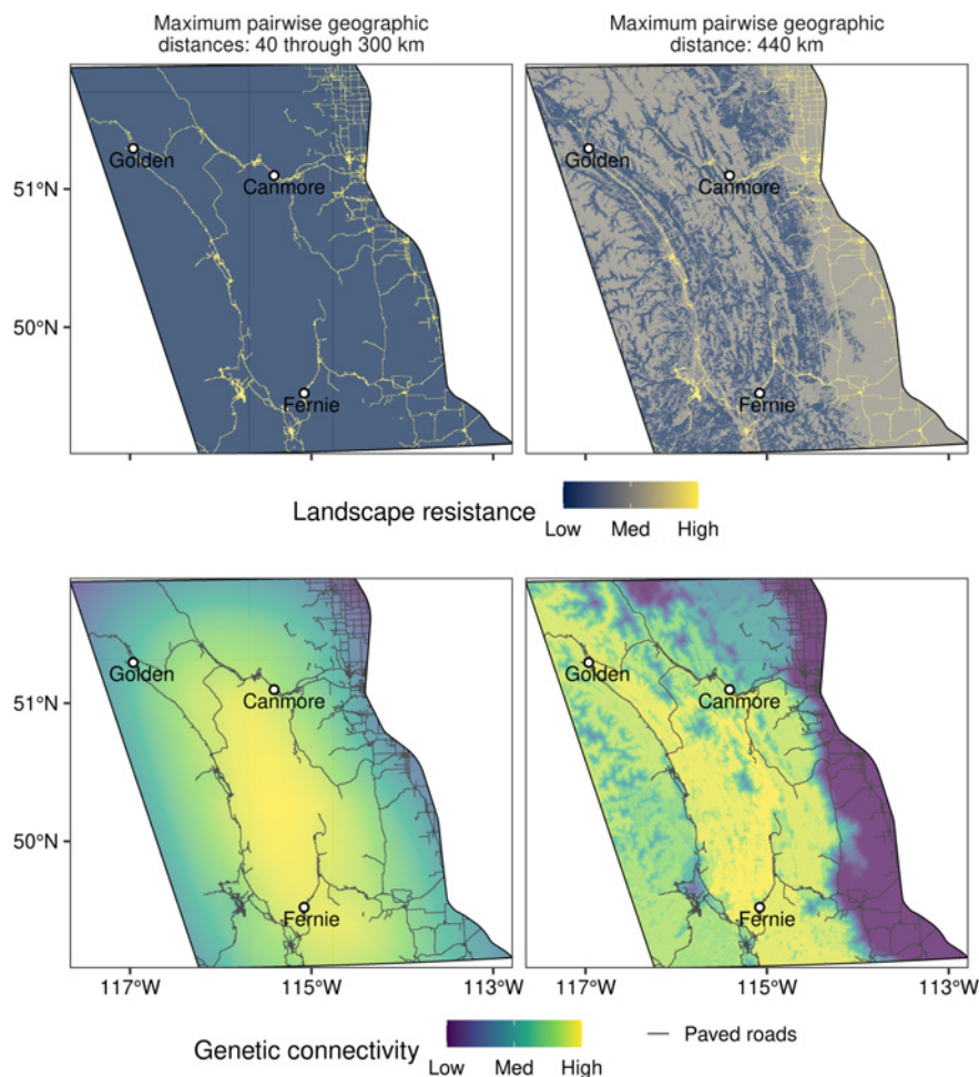
FIGURE 5 Predicted landscape resistance (top) and resistant kernels (bottom) for grizzly bears ( Ursus arctos ) modelled using 1161 genetic samples throughout the southern Canadian Rocky Mountains. [Colour figure can be viewed at wileyonlinelibrary.com ]
