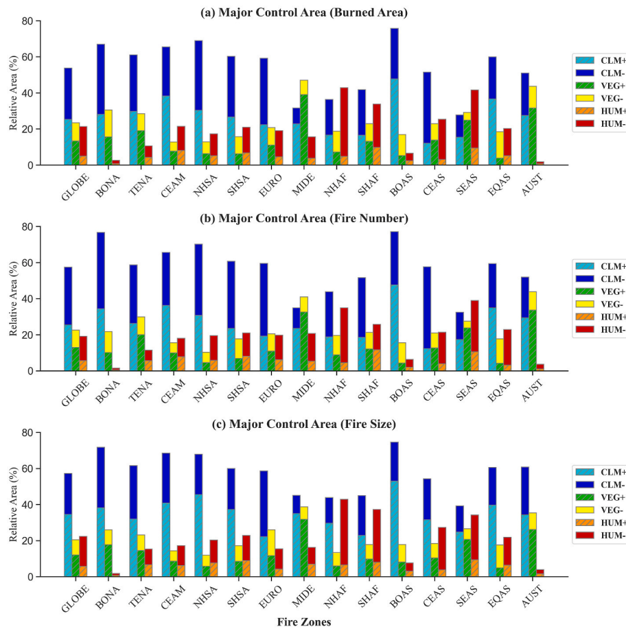
Fig. 7. Comparisons of major fire control areas for burned area, fire number and fire size. Relative areas are the percentage area relative to global burned area (for GLOBE) or total burned area in each fire zone. Six fire control types are seen in Fig. 6.
