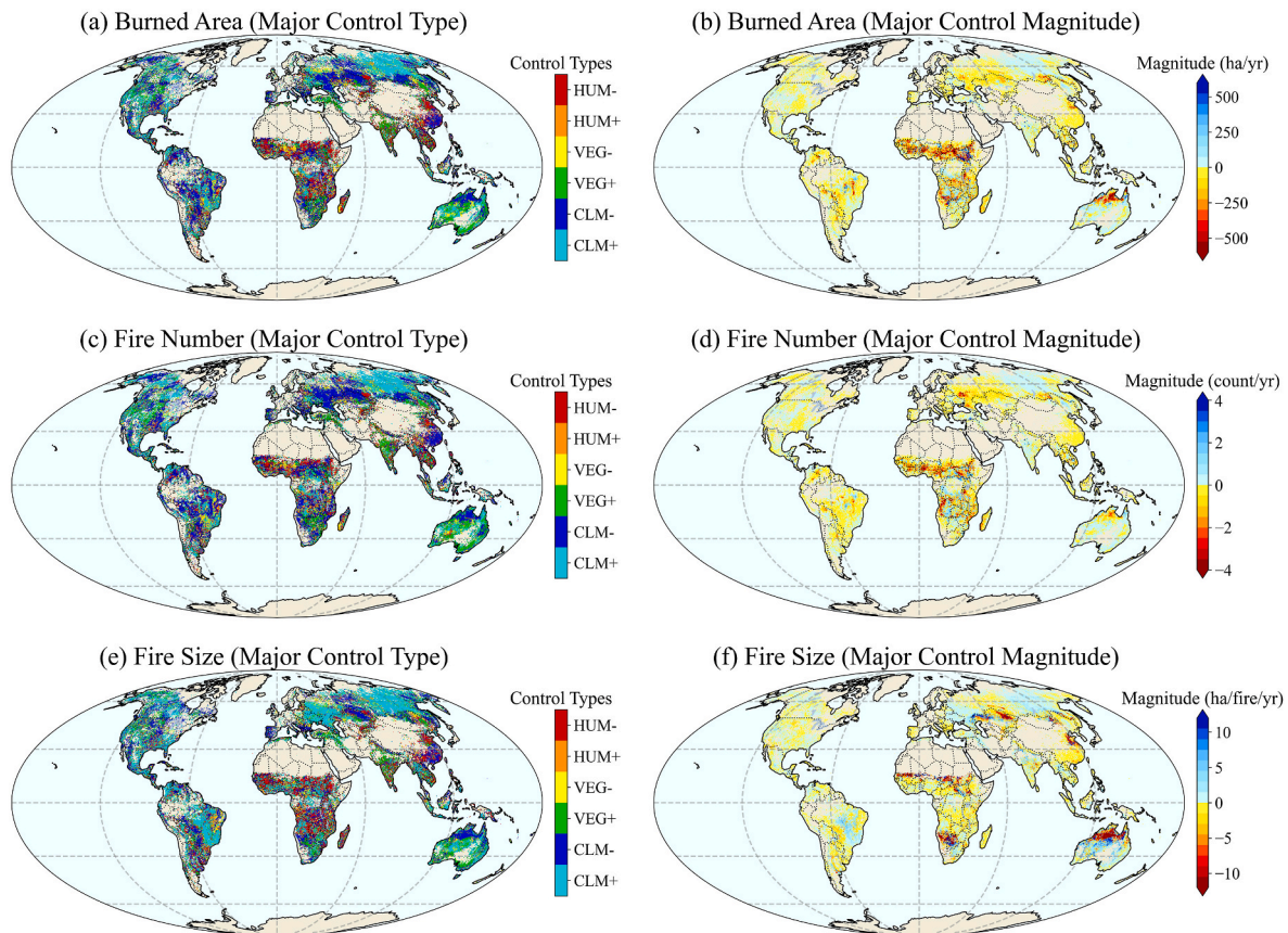
Fig. 6. Spatial patterns of major fire control types and magnitudes for burned area, fire number and fire size. Six fire control types in (a), (c) and (e) are: CLM+ (positive climate control), CLM- (negative climate control), VEG+ (positive vegetation control), VEG- (negative vegetation control), HUM+ (positive human control) and HUM- (negative human control).
