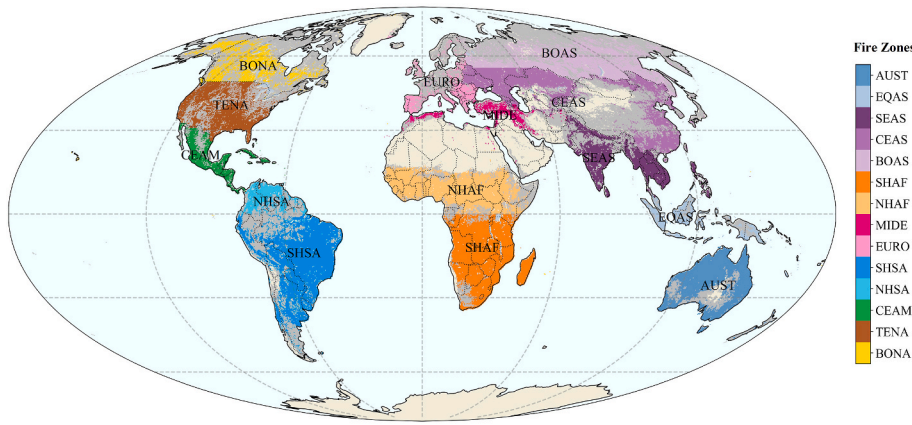
Fig. 1. Fire zones used in this study. Masked land area is unburnable non-vegetated area. The 14 fire zones include: BONA (Boreal North America), TENA (Temperate North America), CEAM (Central America), NHSA (Northern Hemisphere South America), SHSA (Southern Hemisphere South America), EURO (Europe), MIDE (Middle East), NHAf (Northern Hemisphere Africa), SHAF (Southern Hemisphere Africa), BOAS (Boreal Asia), CEAS (Central Asia), SEAS (Southeast Asia), EQAS (Equatorial Asia), and AUST (Australia & New Zealand). Non-vegetated area is labeled as light brown color, while non-fire regions over vegetated area are labeled as gray color. Original source: https://globalfiredata.org/pages/data/#ancillary . (For interpretation of the references to color in this figure legend, the reader is referred to the Web version of this article.)
