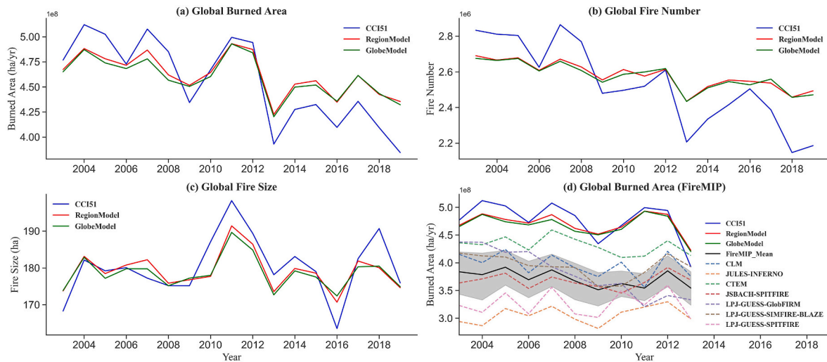
Fig. 3. Evaluations of global fire simulations from the ensemble MLs (GlobeModel & RegionModel) and FireMIP based on the satellite-based fire product from CCI51. 'FireMIP_Mean' in (d) are the mean of seven fire models from FireMIP.
