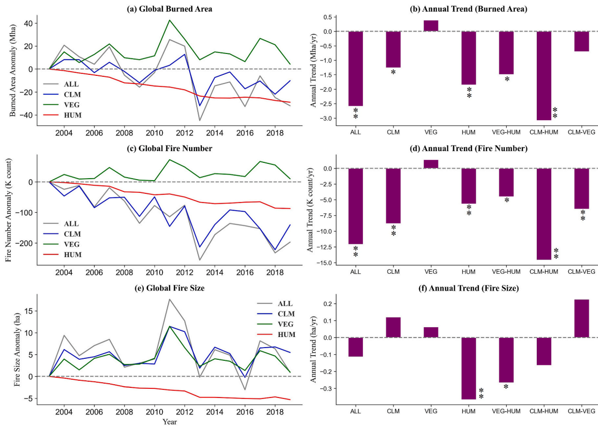
Fig. 5. Effects of climate, vegetation and human controls on annual global burned area, total fire number and averaged fire size. Scenario simulations are seen in Table 1. CLM, VEG, HUM are direct fire controls from climate, vegetation, and human, respectively. ALL is the simulated total controls. VEG-HUM, CLM-HUM and CLM-VEG in (b), (d) and (f) are joint controls from vegetation and human, climate and human, and climate and vegetation, respectively. * p < 0.05 ; ** p < 0.01 .
