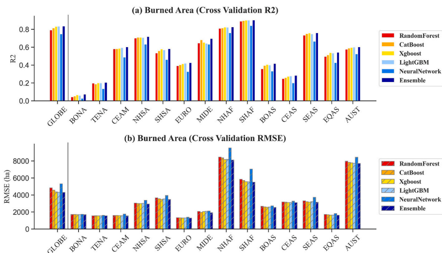
Fig. 2. Grid-level model evaluation for burned area among one global (GLOBE; left side of the vertical line) and 14 regional (right side of the vertical line) ML models based on five-fold cross validation. The abbreviations of fire zones are seen in Fig. 1.
