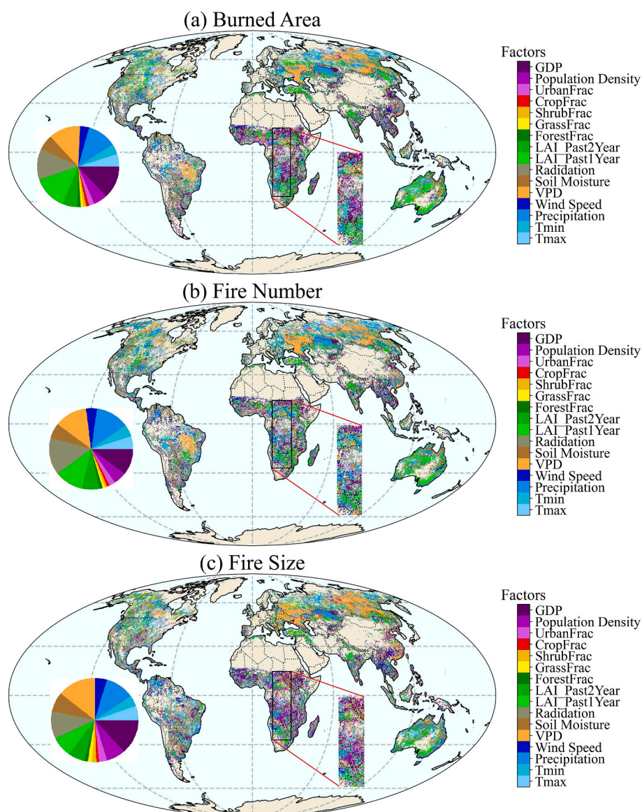
Fig. 8. Dominant factors for major climate, vegetation, and human controls on global burned area (a), fire number (b) and fire size (c). Specific factors are seen in Table S1. The inserted pie chart on the lower left panel is the area proportion for all control factors. The gradient of fire controls in the central Africa from northern to southern hemispheres (marked by black rectangle) is highlighted in each subfigure. The color schemes are used to quantify fire controls from four human factors (purple to red), five vegetation factors (yellow to green) and seven climate factors (gray to yellow and blue). (For interpretation of the references to color in this figure legend, the reader is referred to the Web version of this article.)
