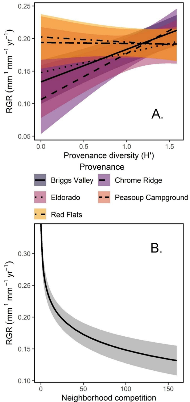
Fig. 2 Relative growth rate (RGR; 1966–1973) as a function of the best-supported model terms of (A) neighborhood provenance diversity, and (B) neighborhood tree competition. The diversity \times provenance interaction effect was approximately 30% the strength of the competition effect
