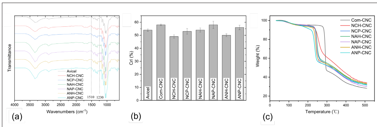
3. (a) Fourier transform infrared (FTIR) spectra; (b) cellulose crystallinity index (CrI) values, and (c) thermogravimetric curves of CNCs isolated from hemp and poplar in comparison to Avicel or commercial CNC (Com-CNC).
