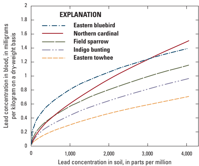
Figure 8. Relations between lead concentration in the soil in the breeding territory and lead concentration in blood for five songbird species at three contaminated sites (Anschutz Mine, Big River floodplain, and Magmont Vent) and two reference sites (Johnson’s Shut-ins State Park and Hawn State Park) in the Southeast Missouri Lead Mining District.
