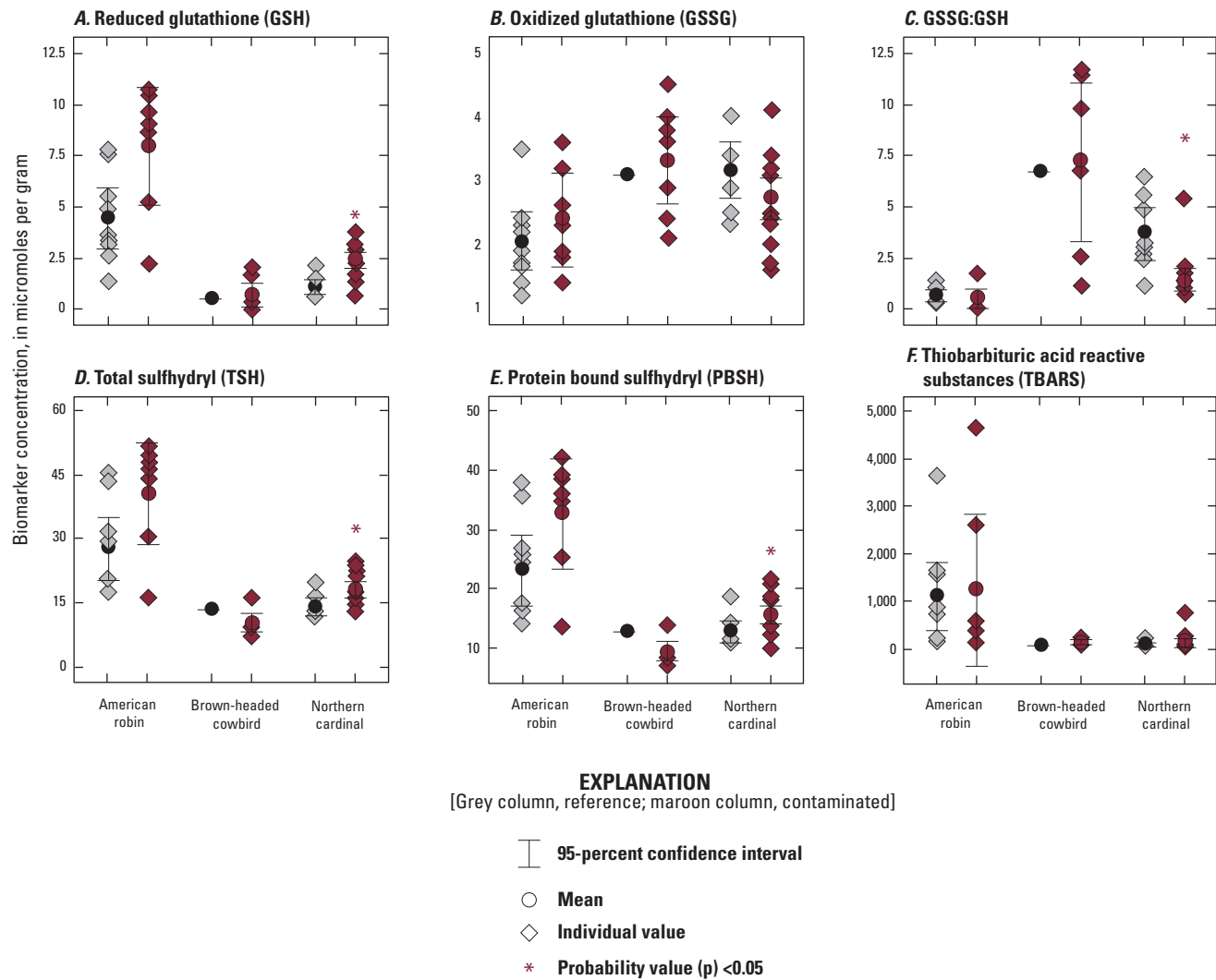
Figure 13. Concentrations of oxidative stress markers in the livers of adult songbirds. A , reduced glutathione (GSH). B , oxidized glutathione (GSSG). C , the ratio of GSSG to GSH (GSSG:GSH). D , total sulfhydryl (TSH). E , protein bound sulfhydryl (PBSH). F , thiobarbituric acid reactive substances (TBARS).
