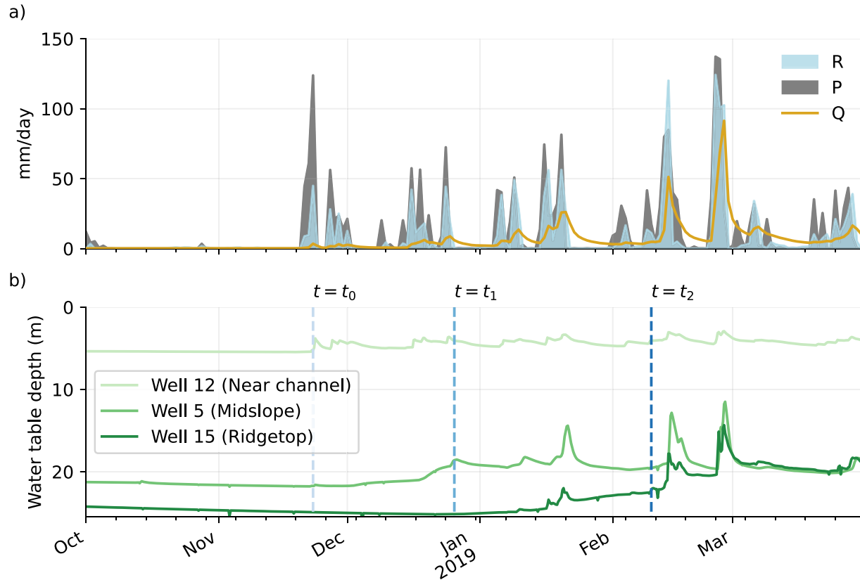
Figure 1. Flow, precipitation, and inferred (positive) groundwater recharge fluxes over the 2019 water year (a). Early season rains do not result in significant recharge because most incoming precipitation is stored in the vadose zone. Groundwater time series at three hillslope positions (b). Near channel groundwater responds fastest due to small vadose zone storage capacity downslope, versus the delayed response at the ridge where storage capacity in the vadose zone is largest. Representative time points ( t_0 , t_1 , t_2 ) correspond to groundwater profiles in Figure 4.
