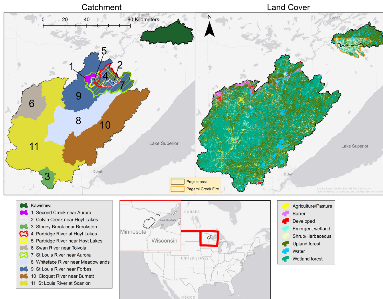
FIGURE 1 Basins and geographic setting.
