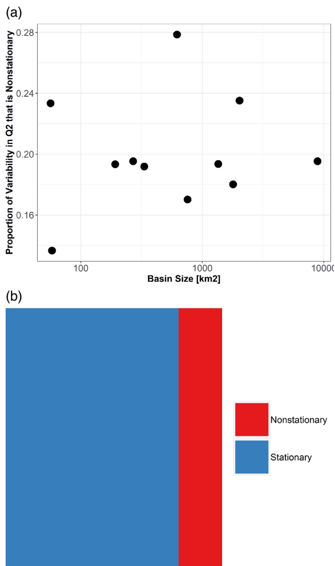
FIGURE 5 (a) Nonstationary component of the Q2, or 50% exceedance probability annual maximum streamflow, that can vary year-to-year, as a proportion of the overall magnitude of the Q2 across all years, for each catchment; (b) overall average across catchments, across years, variability in the Q2 attributable to stationary versus nonstationary processes.
