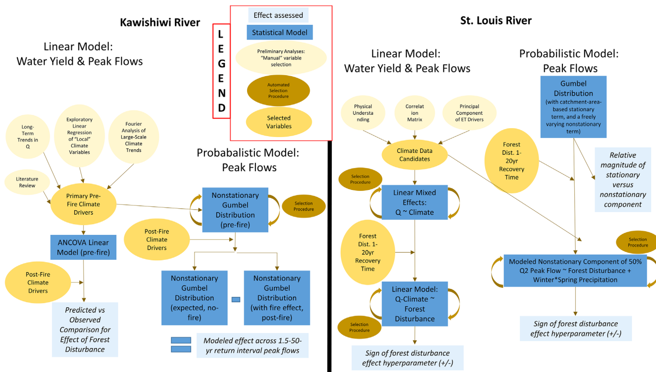
FIGURE 2 Workflow diagram for the analysis techniques used to assess effects of forest disturbance on streamflow on the Kawishiwi and St. Louis River.
