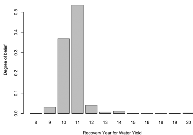
FIGURE 3 Hydrologic recovery year for water yield after forest disturbance, after adjusting for the effects of climate. The degree-of-belief represents how confident we are that the N year recovery year is the best-fitting model for recovery years 1–20. Recovery year represents the number of years after a forest disturbance such as fire, harvest, or windthrow when that parcel no longer influences the water yield regression as a “disturbed” parcel, and was selected according to best-fit of the regression.
