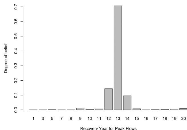
FIGURE 4 Hydrologic recovery year for peak flow after forest disturbance, after adjusting for the effects of climate. The Degree-of-Belief represents how confident we are that the N year recovery year is the best-fitting model for recovery years 1–20. Recovery year represents the number of years after a forest disturbance such as fire, harvest, or windthrow when that parcel no longer influences the peak flow regression as a “disturbed” parcel, and was selected according to the best-fit of the regression.
