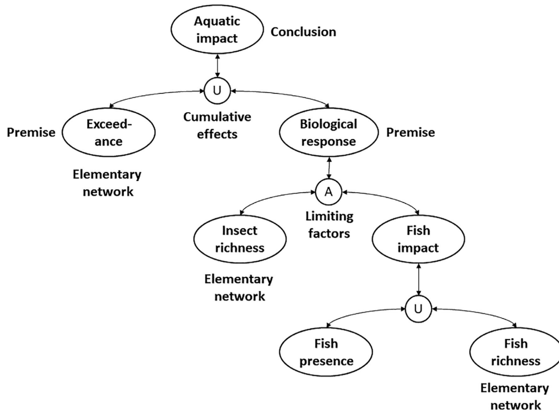
FIGURE 3 Logic to assess S and N deposition impacts. Ovals indicate logic topics, each of which assesses the outcome for the indicated topic. Aquatic impact considers both effects of long-term ecosystem response in terms of steady-state critical loads that determine exceedance and effects of acid neutralizing capacity on short-term biological response. Circles indicate logical operators. The Scenarios section provides additional explanation. A, AND; U, union.
