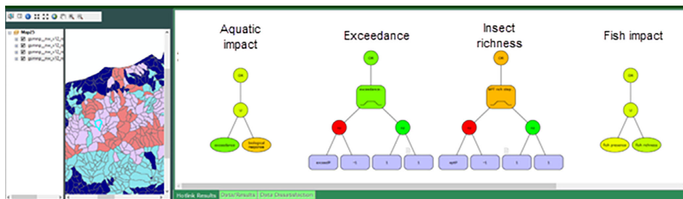
FIGURE 12 Ecosystem Management Decision Support tool for viewing details of NetWeaver logic at the feature level. From left to right, the panes in this figure show: (1) a table-of-contents view of logic topics that have been selected in the tool; (2) a thumbnail map (zoomed in this example) to select a specific feature; and (3) NetWeaver logic topics associated with the table of contents. In the example, a feature has been selected from the map, and the NetWeaver topics are shown in their evaluated state (color coding is for strength of evidence), because the topics are dynamically linked to the selected feature in the map.
