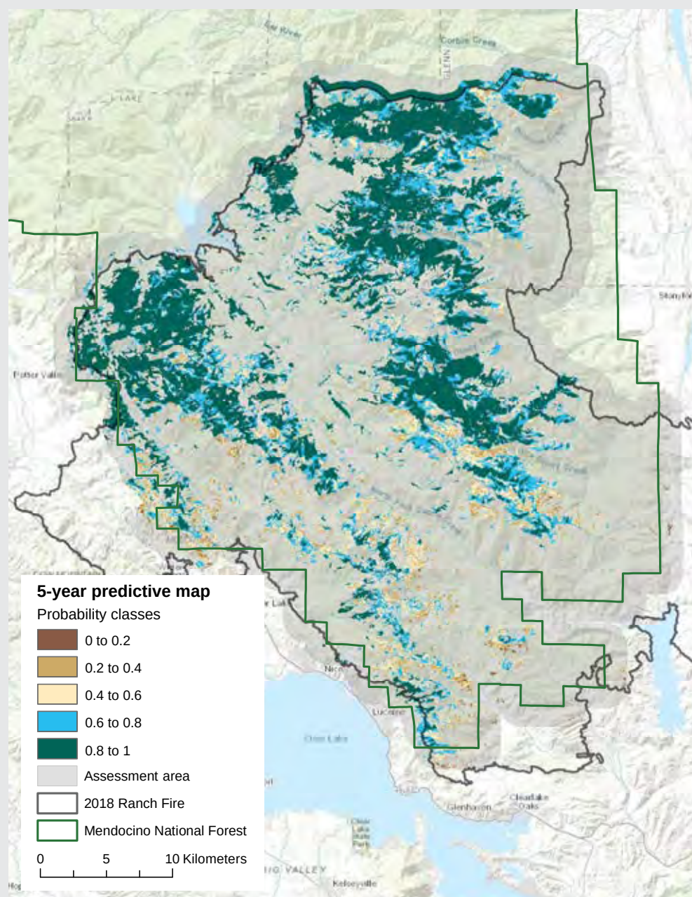
Figure 26—Probability of conifer regeneration (finding at least one regenerating conifer 5 years after fire in a 60-m² area) for yellow pine/mixed-conifer forests in the Ranch Fire analysis area on the Mendocino National Forest. Map by Gabrielle Bohlman.
