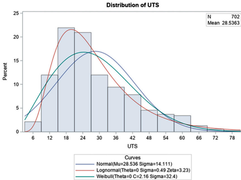
Figure 7. Distribution of ultimate tensile stress (UTS) for 2 × 6—No. 2 southern pine lumber.
