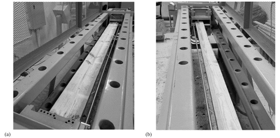
Figure 2. (a) Test setup used to determine tension parallel to the grain properties of 2 × 10 lumber. (b) 2 × 6 southern pine lumber.
