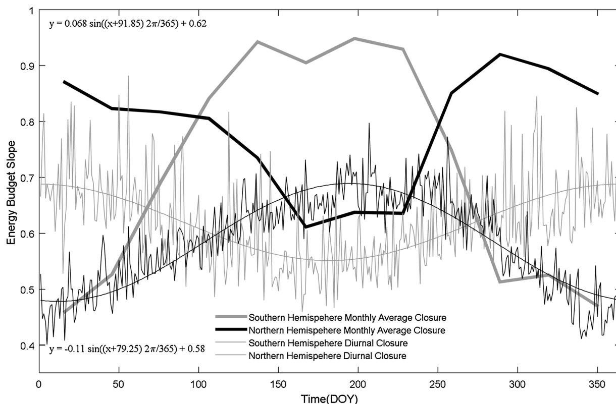
Fig. 7. Variation over an average year in FLUXNET2015 site energy closure, based on regression slope. Site separated by northern hemisphere (black, n = 132 ) and southern hemisphere (grey, n = 27 ). Bold lines shows monthly average regression energy closure at northern (bold black) and southern (bold grey) hemisphere sites.
