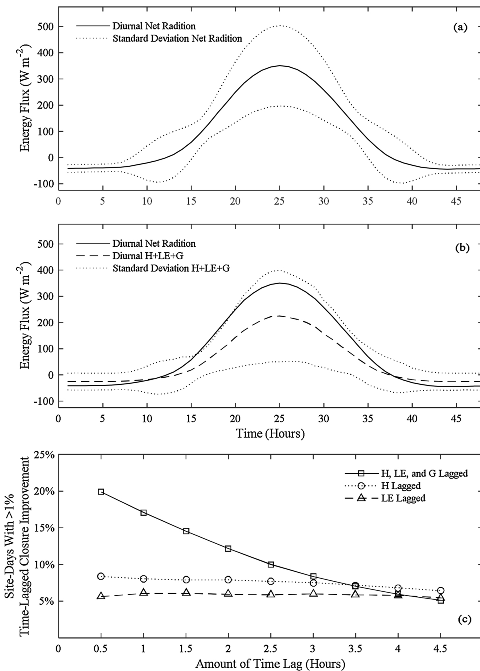
Fig. 8. Diurnal net radiation and its standard deviation (a) and diurnal sum of surface heat fluxes ( H + LE + G ) and its standard deviation (b), with diurnal net radiation plotted as a reference, across the entire FLUXNET2015 site-days that show a 1% or better improvement in energy closure with all energy fluxes, sensible and latent heat fluxes lagged in time (c).
