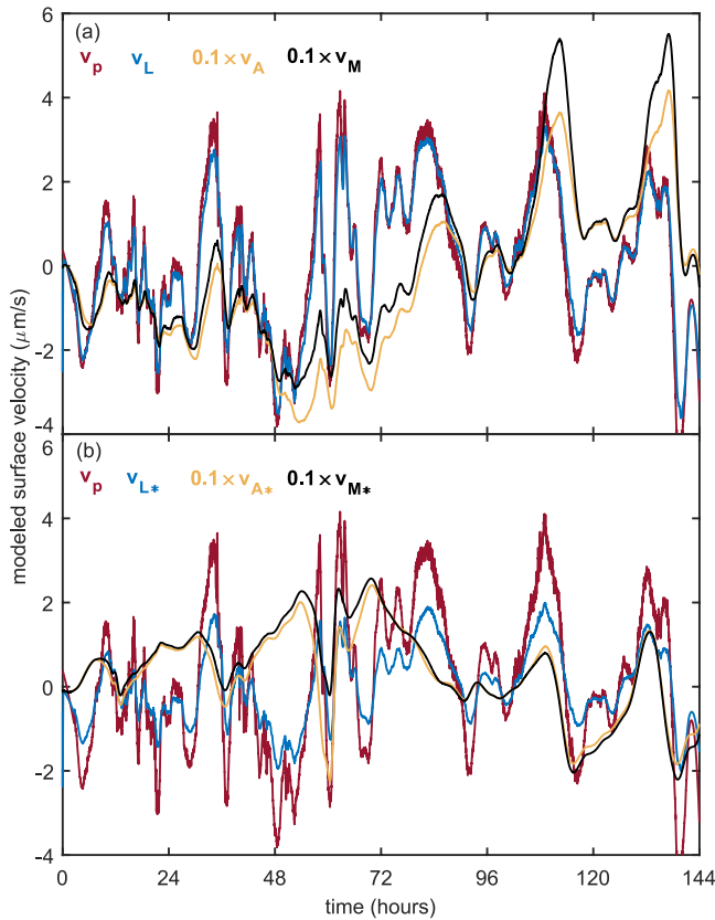
Figure 4. (a) Estimates of low frequency advective velocities induced by pressure dynamics only using the Linear model ( v_L , Equation 7), the Muskat model ( v_M , Equation 10), and the Approximate model ( v_A , Equation 11) for 14–20 June 2012. v_p from the conservation of mass (COM), Equation 19 is included for comparison. (b) Estimates of low frequency advective velocities induced by pressure, temperature, and soil moisture dynamics combined using the Linear model ( v_{L*} , Equation 13), the Muskat model ( v_{M*} , Equation 14), and the Approximate model ( v_{A*} , Equation 15) for 14–20 June 2012. v_p from the COM, Equation 19 is included for comparison.
