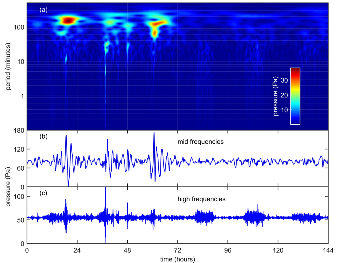
Figure 5. (a) Wavelet decomposition of the 14–19 June 2012, soil surface pressure time trace using the Morlet wavelet after removing the low frequencies, that is, all frequencies with periods longer than 5 hr. (b) Filtered mid frequency (periods between 0.5 and 5 hr) surface pressure time series. (c) Filtered high frequency (periods between 1 s and 0.5 hr) surface pressure time series. Three (self-identified) inertia-gravity waves occur each day during the first 72 hr (14–16 June). Wave periods of these events (panel (b)) were between about 2.1 and 2.5 hr with maximum amplitudes between approximately 30 and 70 Pa. Rain fell about hour 60 (mid-day 16 June). The daily pulses of high frequency surface pressure, panel (c), during the last 72 hr (17–19 June) are interpreted here as the diel cycle in turbulence, suggesting that the three wave events (panel (b)) intensify the diel cycle of turbulence. Finally, in addition to the inertia-gravity wave the second day (panel (b)) appears to include a slightly higher frequency gravity wave event centered at about 48 hr.
