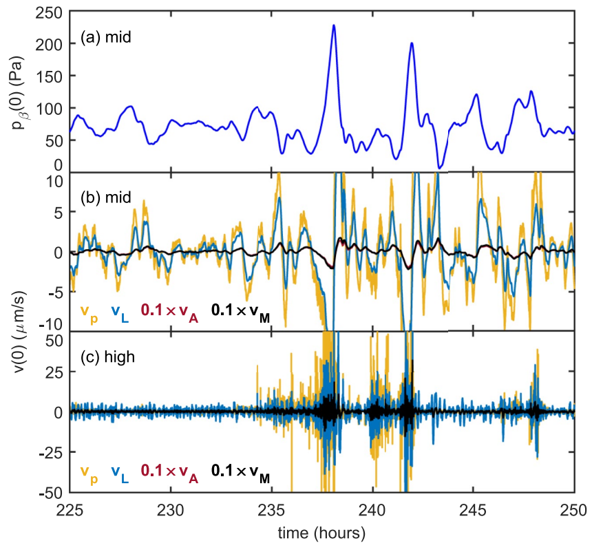
Figure 8. (a) Last 25 hr of the October 2012 soil surface pressure time series. The two pressure events centered at approximately 237 and 243 hr are interpreted here as solitons and they correspond to the rightmost (complex) “bright spot” on Figure 7a. (b) Last 25 hr of the modeled (b) mid frequency soil surface velocities and (c) high frequency soil surface velocity time series. Because v_A \leq v_M , v_A is obscured by v_M in panel (c). All velocities highlight the impact that the solitons, shown in panel (a), can have on the soil advective velocity field. Note the episodic nature of the high frequency velocities, their (relatively) strong association with the soliton events, and that the high frequency velocities are often about a factor of two or more greater in magnitude than the mid-frequency velocities.
