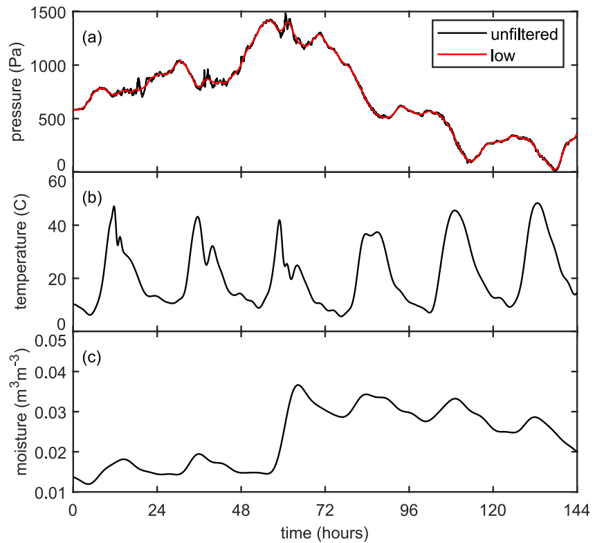
Figure 1. Model drivers (or surface forcing functions) for the 14–20 June 2012 simulation. (a) The black line is the observed 1 Hz surface pressure data, p_\beta(t, 0) , which has had enough of the background pressure removed to ensure all data are \geq 0 . The red line is the numerically filtered low frequency component of the surface pressure and includes only those data with periods \geq 5 hr. (b) 1 Hz temperature forcing function, T_\beta(t, 0) , interpolated from the observed 5 min averages of the soil surface temperatures. The frequency content of this forcing is limited almost exclusively to low frequencies with only a small component of mid frequency content (i.e., periods between 0.5 and 5 hr). (c) 1 Hz soil moisture forcing function, \theta_\beta(t, 0) , interpolated from the observed 5 min averages of the 2-cm volumetric soil moisture. This forcing is exclusively low frequency because the mid and high frequency content (i.e., with periods between 1 s and 0.5 hr) was low amplitude noise that has no influence on the numerical results.
