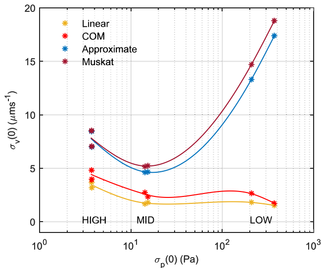
Figure 9. Summary plot of the response, \sigma_v(0) , versus the forcing, \ln(\sigma_p(0)) , for the June and October study periods as a function of frequency band for the conservation of mass approach, the linear model and the two nonlinear models. Low frequencies refer to atmospheric pressure variations with periods \geq 5 hr, mid frequencies have periods between 0.5 and 5 hr, and high frequencies have periods between 1 s and 0.5 hr. Given that \sigma_p(0) increases fairly strongly with decreasing frequency this plot can also be interpreted as a crude description of the different models' spectral response.
