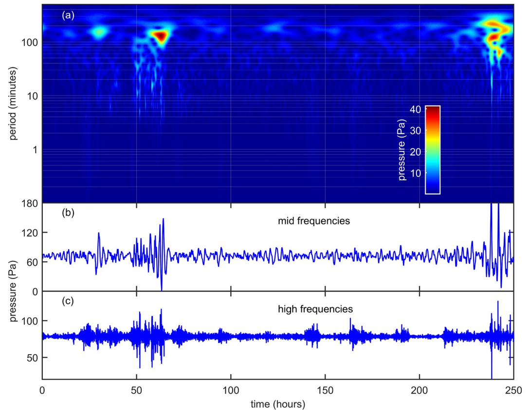
Figure 7. (a) Wavelet decomposition of the 2–13 October 2012, soil surface pressure time trace using the Morlet wavelet after removing the low frequencies, that is, all frequencies with periods longer than 5 hr. (b) Filtered mid frequency (periods between 0.5 and 5 hr) surface pressure time series. (c) Filtered high frequency (periods between 1 s and 0.5 hr) surface pressure time series. Two (self-identified) inertia-gravity waves occur each day between (approximately) 24 and 72 hr (3 and 4 October). Wave periods of these two waves, panel (b), were between about 2.2 and 2.6 hr with maximum amplitudes between approximately 20 and 60 Pa. A pair of atmospheric solitons (also self-identified) appear as two positive spikes in panel (b), the mid-frequency time series, during the last 24 hr (13 October). The amplitudes of these two events are between about 80 and 110 Pa with durations between about 1.6 and 2 hr. Rain fell just after hour 240 (mid-day 13 October). Similar to the June study period (Figure 5c), the diel cycle of turbulence is also present during the October period and again both the inertia-gravity waves and the solitons appear to intensify the high frequency turbulent surface pressure perturbations.
