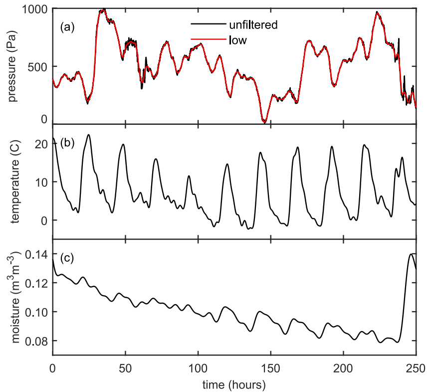
Figure 2. Model drivers (or surface forcing functions) for the 2–13 October 2012 simulation. (a) The black line is the observed 1 Hz surface pressure data, p_\beta(t, 0) , which has had enough of the background pressure removed to ensure all data \geq 0 . The red line is the numerically filtered low frequency component of the surface pressure and includes only those data with periods \geq 5 hr. (b) 1 Hz temperature forcing function, T_\beta(t, 0) , interpolated from the observed 5 min averages of the soil surface temperatures. The frequency content of this forcing is limited almost exclusively to low frequencies with only a small component of mid frequency content (i.e., periods between 0.5 and 5 hr). (c) 1 Hz soil moisture forcing function, \theta_\beta(t, 0) , interpolated from the observed 5 min averages of the 2-cm volumetric soil moisture. This forcing is exclusively low frequencies because the mid and high frequency content (i.e., with periods between 1 s and 0.5 hr) was low amplitude noise that has no influence on the numerical results.
