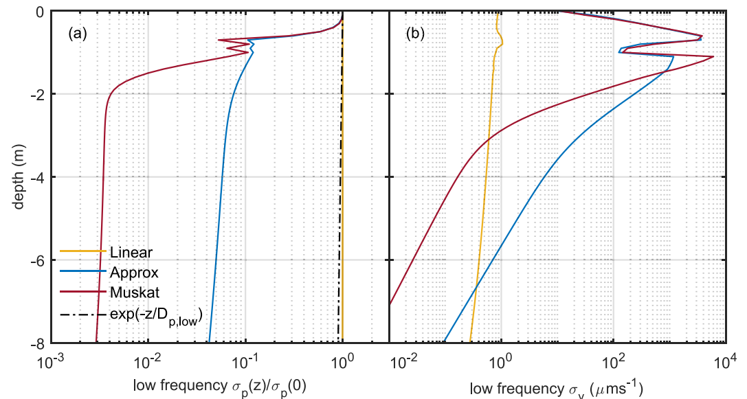
Figure 12. Low frequency (June 2012) modeled profiles in the top 8 m of the model domain with heat and moisture dynamics included (i.e., Equations 13–15). The conservation of mass approach is identified by the expression \exp(-z/D_p) , where D_p = 75 \text{ m} for the low frequencies. Panel (a) shows the modeled vertical profiles of the normalized standard deviation of pressure and panel (b) the standard deviation of advective velocities.
