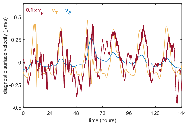
Figure 3. Estimates of low frequency advective velocities induced by pressure, temperature and soil moisture dynamics using the conservation of mass approach (Equations 19–21) for 14–20 June 2012. As discussed in the text, the soil temperature and moisture forcing functions, and therefore, v_T and v_\theta as well, are for all numerical purposes low frequency only.
