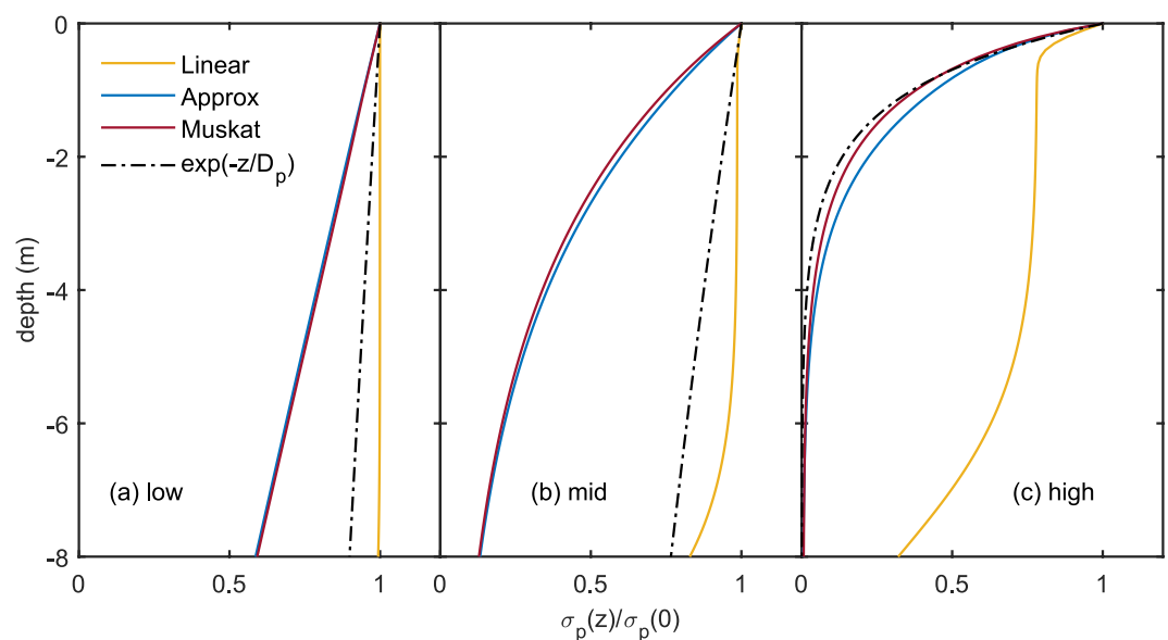
Figure 10. Modeled vertical profiles of the normalized standard deviation of pressure for the top 8 m of the model domain during the 14–20 June 2012 study period. The conservation of mass approach is identified by the expression \exp(-z/D_p) , where D_p = 75 m for the low frequencies, for mid frequencies D_p = 30 m, and D_p for the high frequencies is 1 m.
