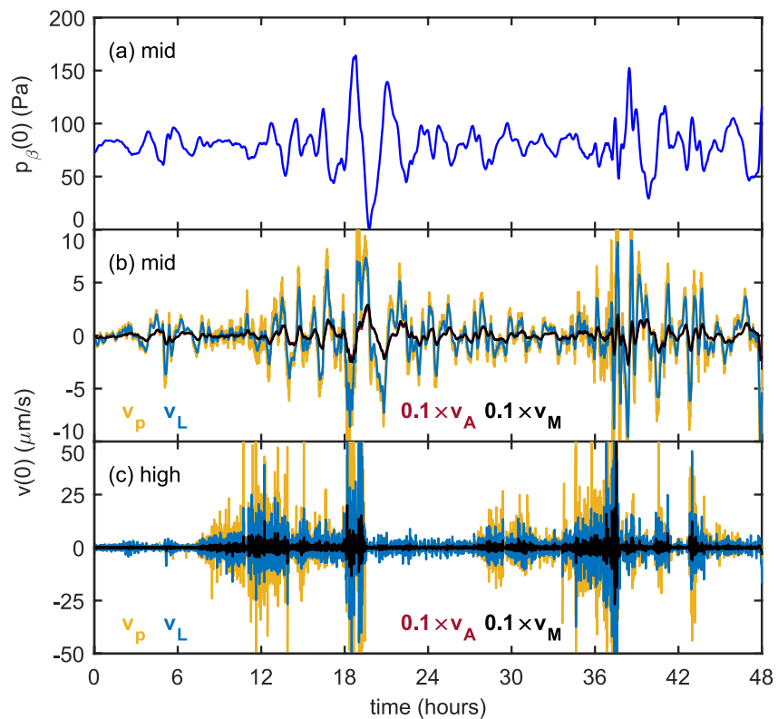
Figure 6. (a) First 48 hr of the June 2012 mid-frequency soil surface pressure time series. The surface pressure perturbations between approximately 16 and 24 hr and the more complex signal between about 36 and 48 hr are interpreted here as an inertia-gravity wave events. These two wave events coincide with the leftmost (first and second) “bright spots” on Figure 5a. (b) First 48 hr of the modeled June 2012 mid frequency soil surface velocities and (c) first 48 hr of the modeled high frequency surface velocities. Because v_A \leq v_M , v_A is obscured by v_M in panel (c). All velocities highlight the impact that the inertia-gravity waves, shown in panel (a), can have on the soil advective velocity field. Note the episodic nature of the high frequency velocities, their (at least partial) association with the wave events, and that the high frequency velocities are often about an order of magnitude greater than the mid-frequency velocities.
