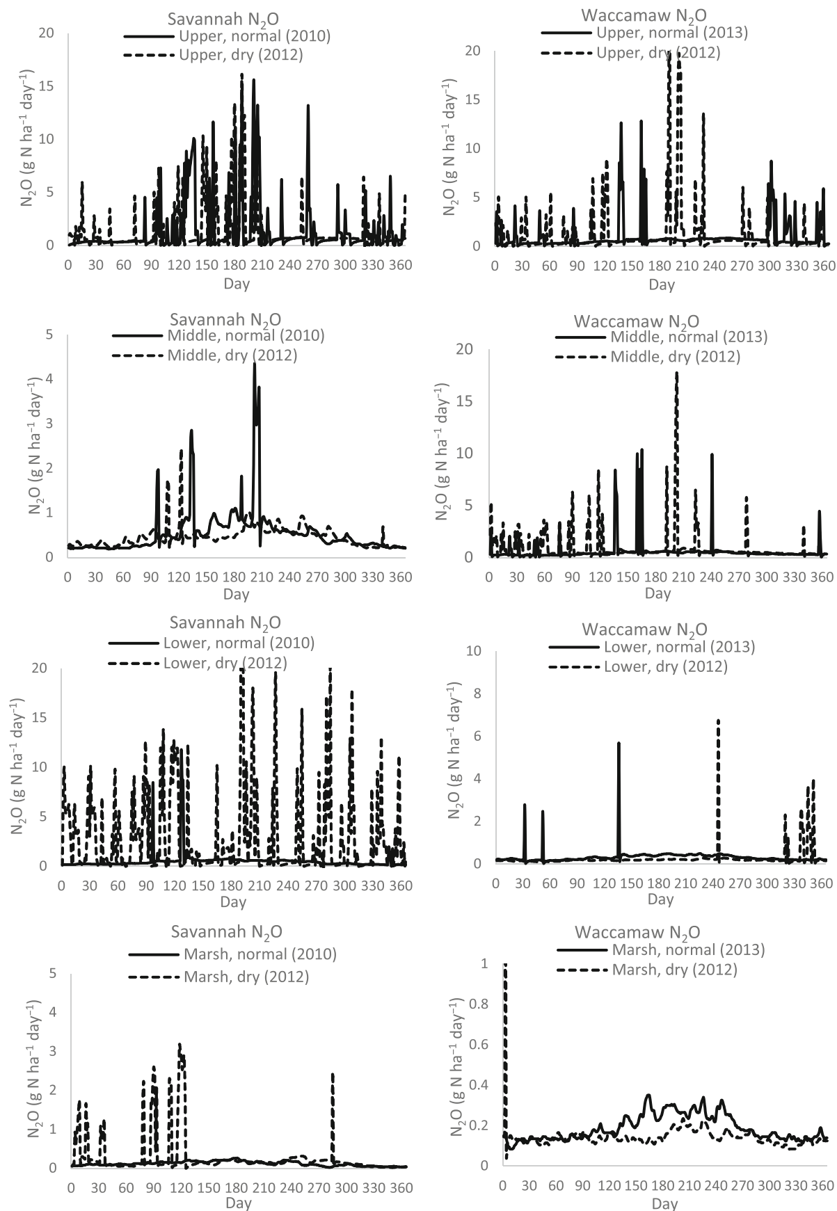
FIGURE 7 Simulated daily soil N_2O emissions under the normal and drought conditions at the upper (top row), middle (second row), lower (third row) forest and oligohaline marsh (fourth row) sites along the Savannah and Waccamaw rivers.
