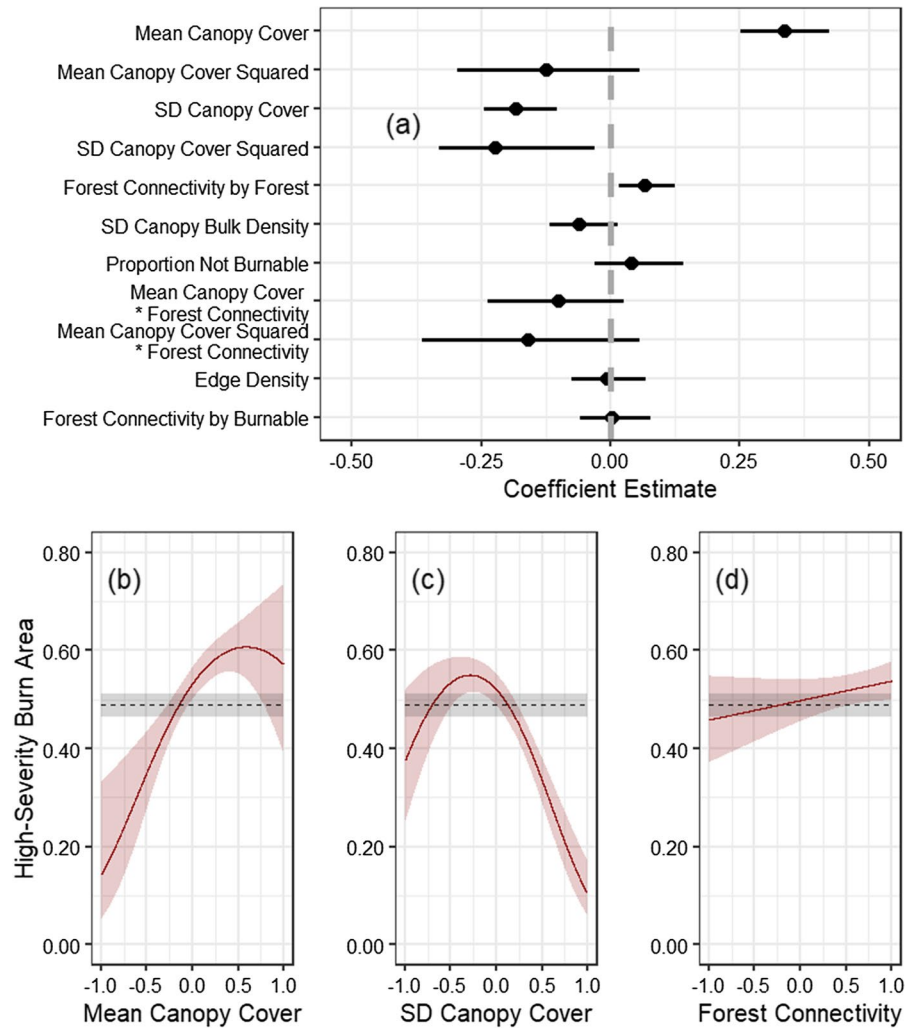
Fig. 2 Responses of the 95th percentile of high-severity burned forest area (referred to as high-severity burn area in the manuscript text) to forest fuel conditions from 2001 to 2020. The standardized coefficients and 95% confidence intervals for all variables included in the model (a), and (b–d) the predicted 95th percentile high-severity burned forest area on the y-axis, modeled as a function of each predictor variable (scaled) for which the 95% confidence interval of the standardized coefficient did not include zero: mean canopy cover (b), standard deviation in canopy cover (c), and forest connectivity (d). Gray dashed lines and gray shading shows the null model and 95% confidence intervals of the 95th percentile high-severity burned forest area, and red lines and red shading shows the predicted response and 95% confidence interval of the response of the 95th percentile of high-severity burned forest area to each scaled predictor variable
