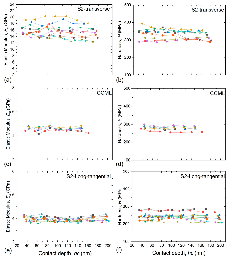
Figure 4. Elastic modulus and hardness of wood cell walls obtained from individual nanoindentations. (a,b) S2 layer in the transverse orientation; (c,d) CCML in the transverse orientation; (e,f) S2 layer in the longitudinal–tangential orientation. Each colored curve represents the complete multiloading segment of a nanoindentation.
