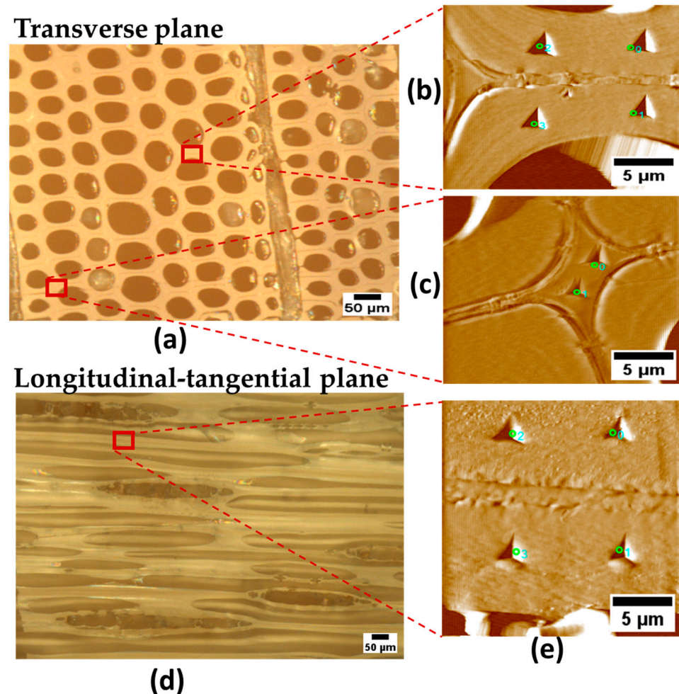
Figure 3. Cutting planes in radiata pine wood. (a) Transverse plane with nanoindentations on (b) S2 layer and (c) CCML, (d) Longitudinal–tangential plane with nanoindentations on (e) S2 layer.
