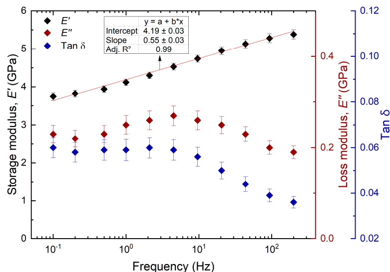
Figure 7. Viscoelastic properties of the S2 layer in the longitudinal–tangential plane. Error bars are the standard error.
