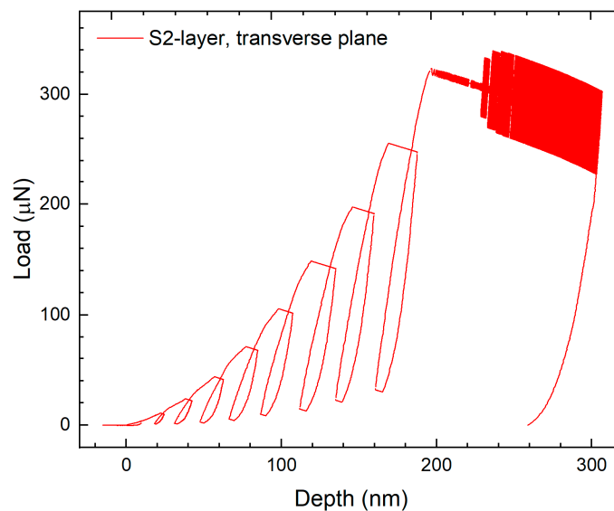
Figure 2. Load depth trace of a quasistatic and dynamic experiment on the transverse plane in the S2 layer of radiata pine wood cell wall.
