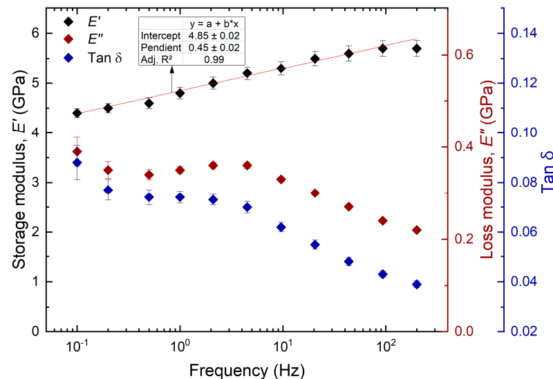
Figure 6. Viscoelastic properties of the CCML in the transverse plane. Error bars are the standard error.
