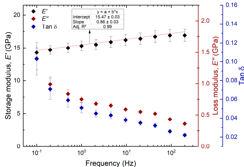
Figure 5. Viscoelastic properties of the S2 cell wall layer in the transverse plane. Error bars are the standard error.
