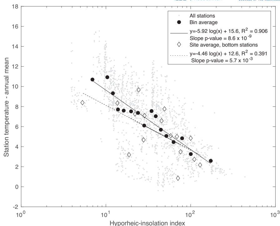
FIGURE 7 Temperature difference, \Delta T_{sa} , versus hyporheic insolation index, H_{in} , for all station-days (bottom, middle, and top) from stratified column-days, 1368 station-days in all, as well as bin-averaged (solid circles) and site-averaged (hollow diamond) values.
