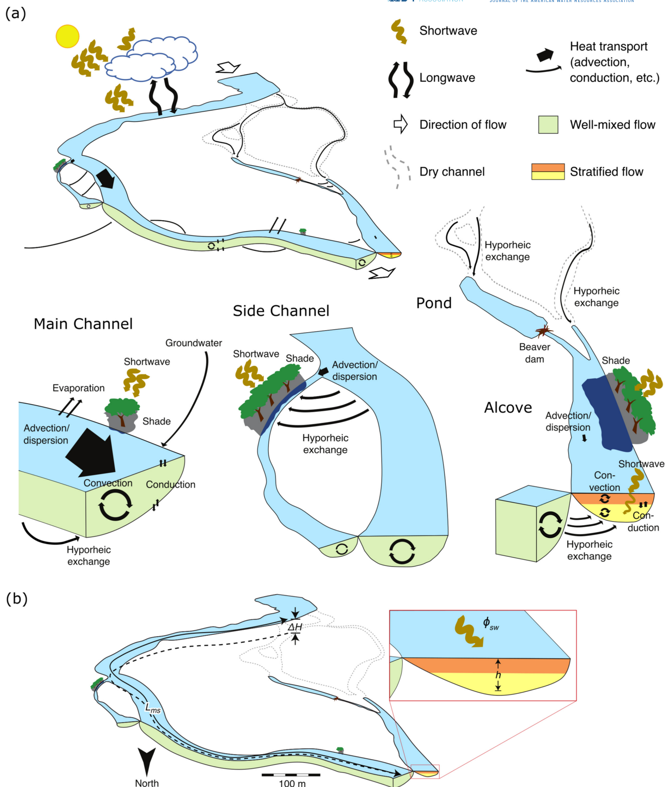
FIGURE 1 Schematic diagram, based on an oblique aerial photograph of the Willamette River, Oregon, of the heat budget (a) and key variables in dimensional analysis (b). (a) In water bodies with large enough flow velocities, advection and dispersion dominate local heat transport and, with convective mixing, make water temperature nearly uniform; bare-gravel surfaces are abundant, and channel banks may have sparse riparian vegetation, which shades relatively little of wide channels. In ponds and alcoves cut off from surface flow, stratification into shallow and deep layers prevents mixing, and results in attenuation of shortwave radiation to deep layers, where hyporheic or groundwater inputs may dominate temperature. (b) Key variables in dimensional analysis include shortwave radiation, \phi_{sw} , mainstem length, L_{ms} , and change in head along the hydraulic flowpath, \Delta H .
