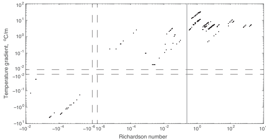
FIGURE 6 Temperature gradient versus Richardson number for each column-day at sites with applicable velocity measurements. Positive and negative values of both are shown and separated by dashed lines. Vertical gray line indicates the critical value (0.25) of Richardson number. Below this threshold, lower values indicate higher degrees of turbulence.
