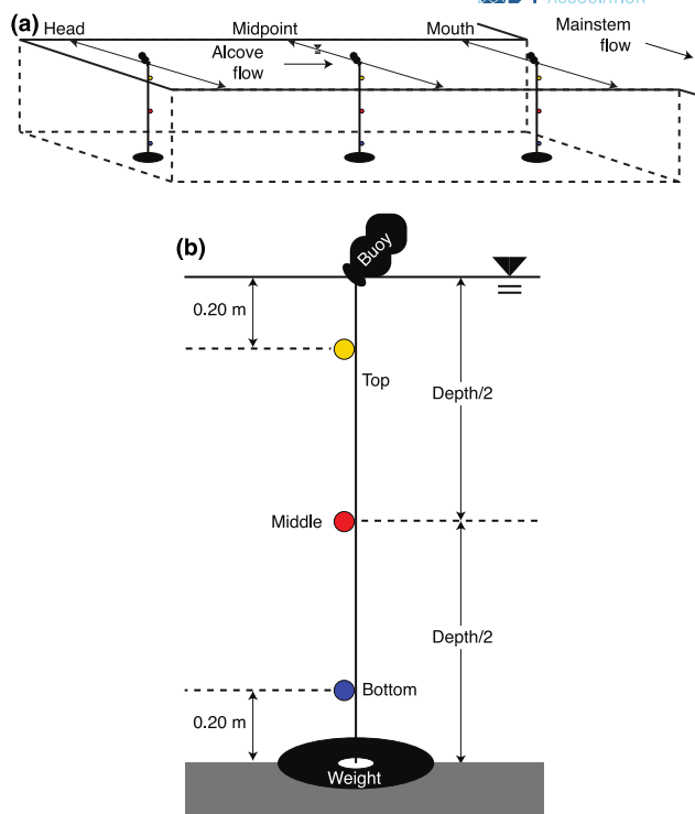
FIGURE 3 Temperature logger deployment scheme for off-channel sites: (a) longitudinal positions of vertical columns at the head, midpoint, and mouth of secondary channel features, and (b) vertical positions of loggers at three stations, bottom, middle, and top, along a cord suspended from a buoy and held in place by a weight (3 kg). Arrows indicate direction of flow in the main channel and in the alcove channel/alcove/pond.
